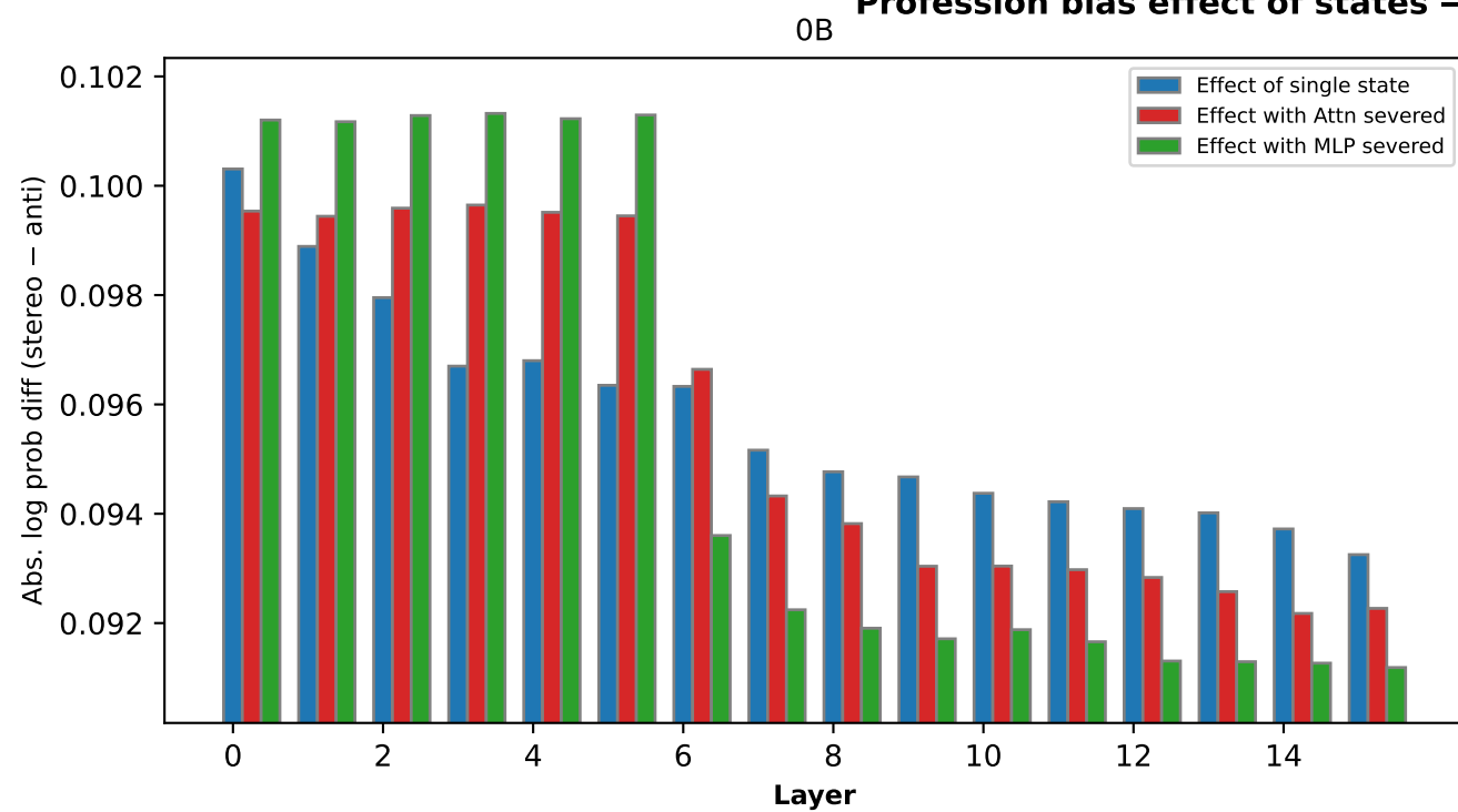
Profession bias effect of states — OLMo-2-0425-1B (all checkpoints)
