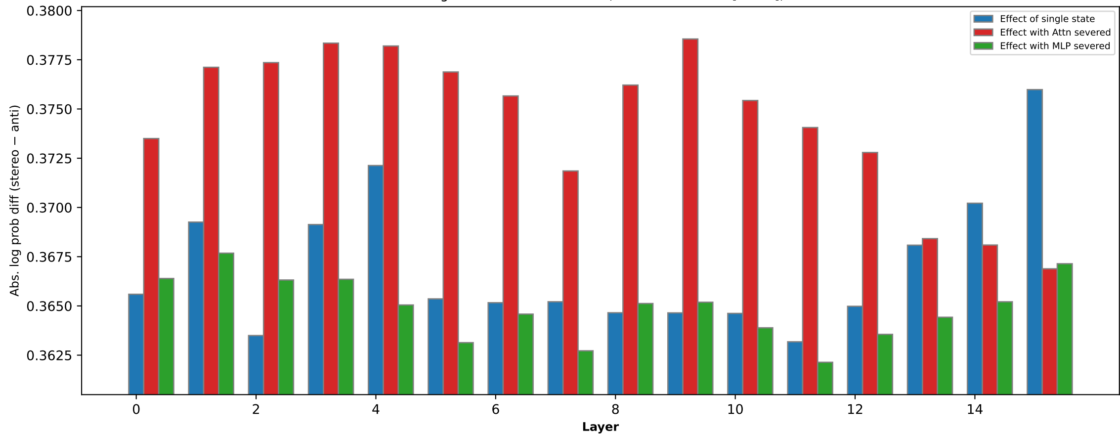
Religion bias effect of states (OLMo-2-0425-1B [s2-3B])
