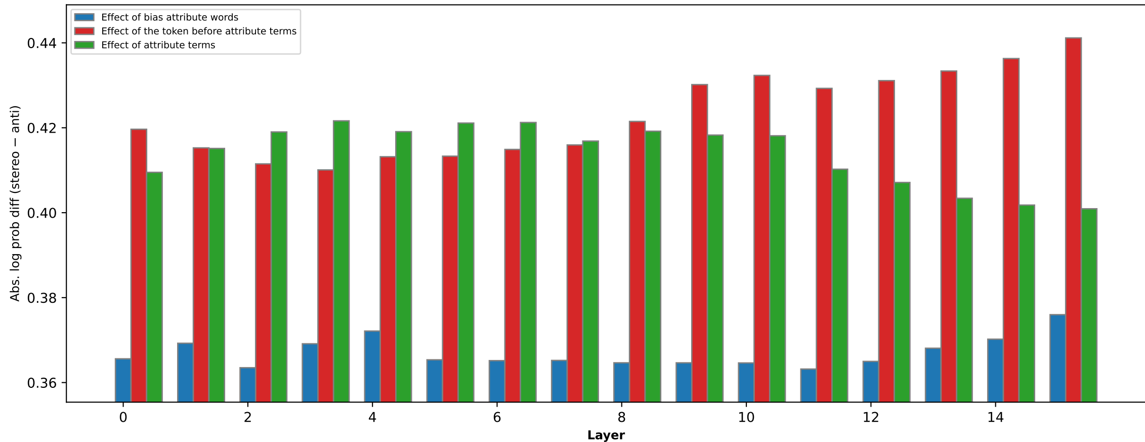
Religion bias effect of different words (OLMo-2-0425-1B [s2-3B])
