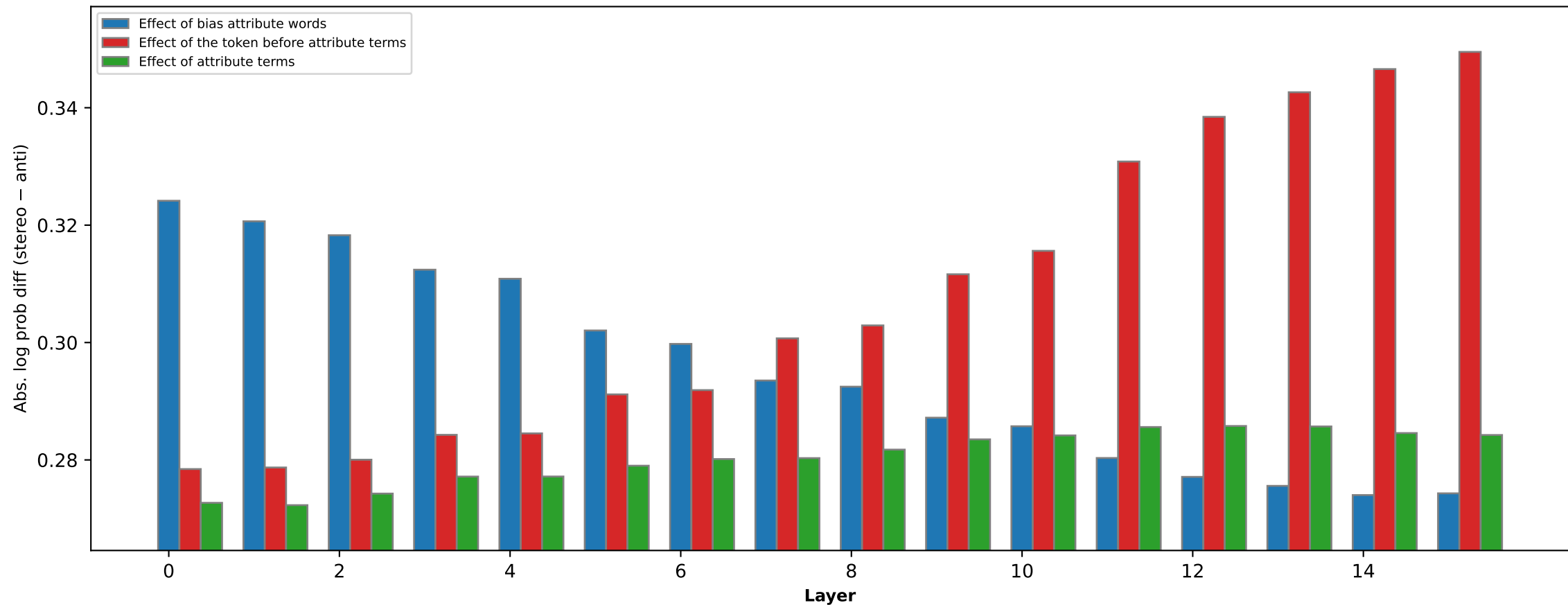
Profession bias effect of different words (OLMo-2-0425-1B [s2-51B])
