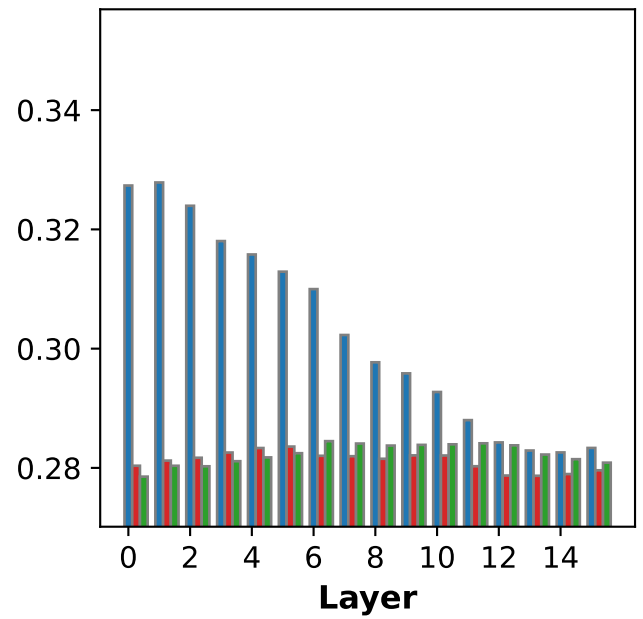
(f) Profession bias effect of different words (OLMo-2-0425-1B)
