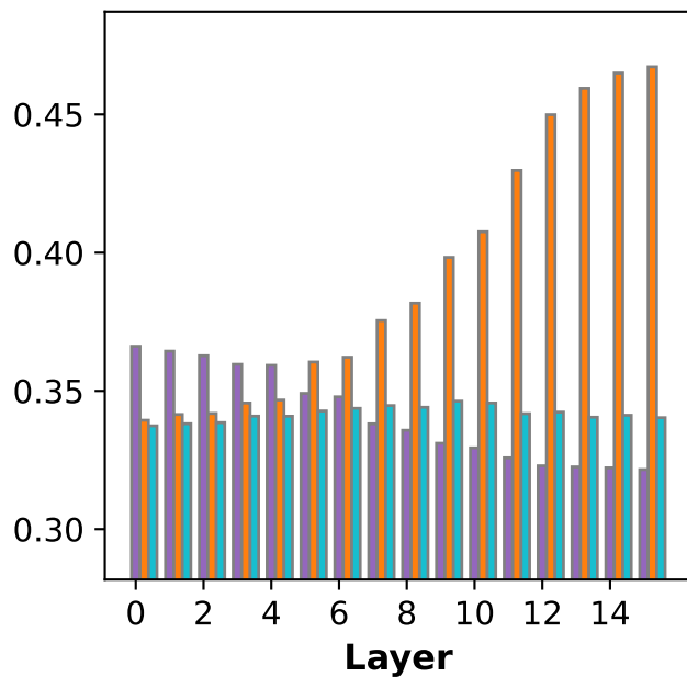
(k) Race bias effect of different words (OLMo-2-0425-1B-Instruct)
