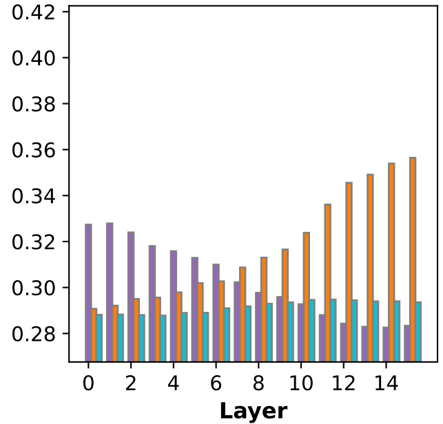
(i) Profession bias effect of states (OLMo-2-0425-1B-Instruct)
