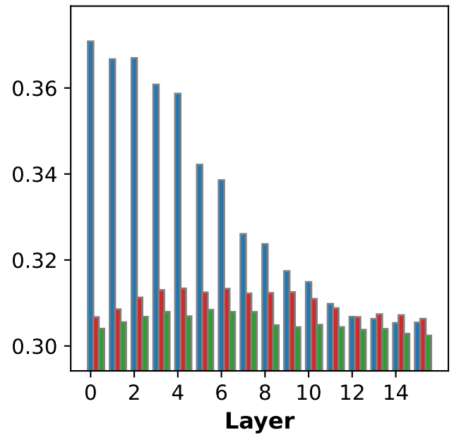
(l) Profession bias effect of different words (OLMo-2-0425-1B-Instruct)
