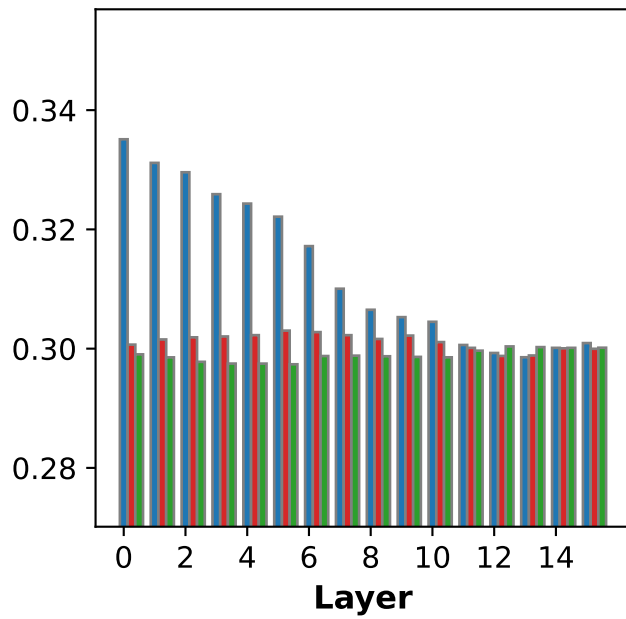
(e) Race bias effect of different words (OLMo-2-0425-1B)
