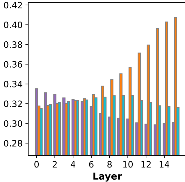
(h) Race bias effect of states (OLMo-2-0425-1B-Instruct)
