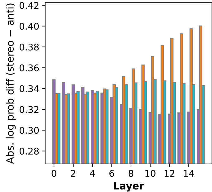
(g) Gender bias effect of states (OLMo-2-0425-1B-Instruct)
