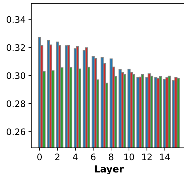
(c) Profession bias effect of states (pythia-1b)
