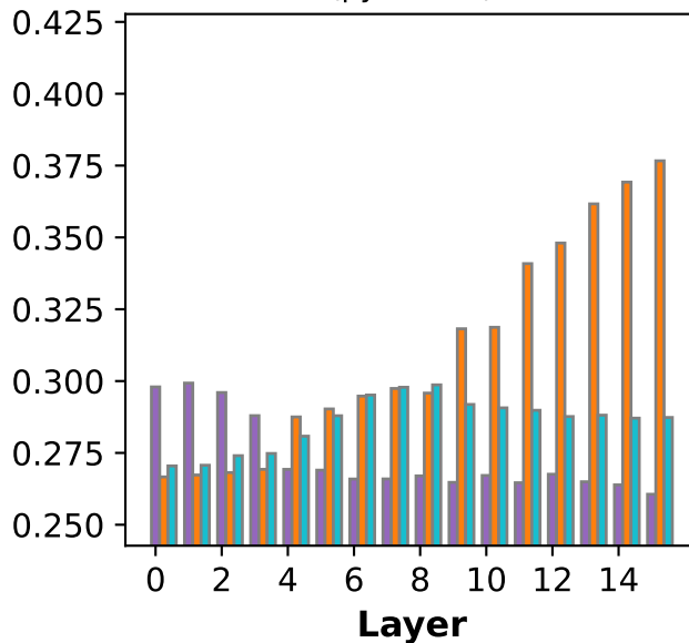
(e) Race bias effect of different words (pythia-1b)
