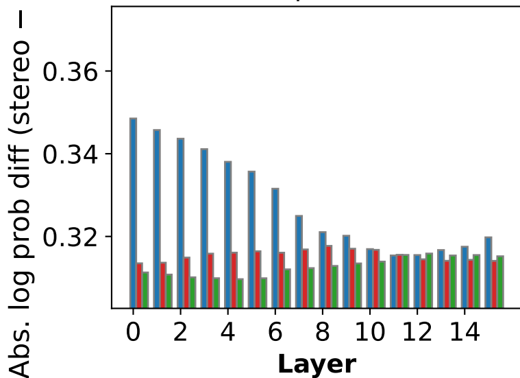
(a) OLMo-2-0425-1B (pre)
