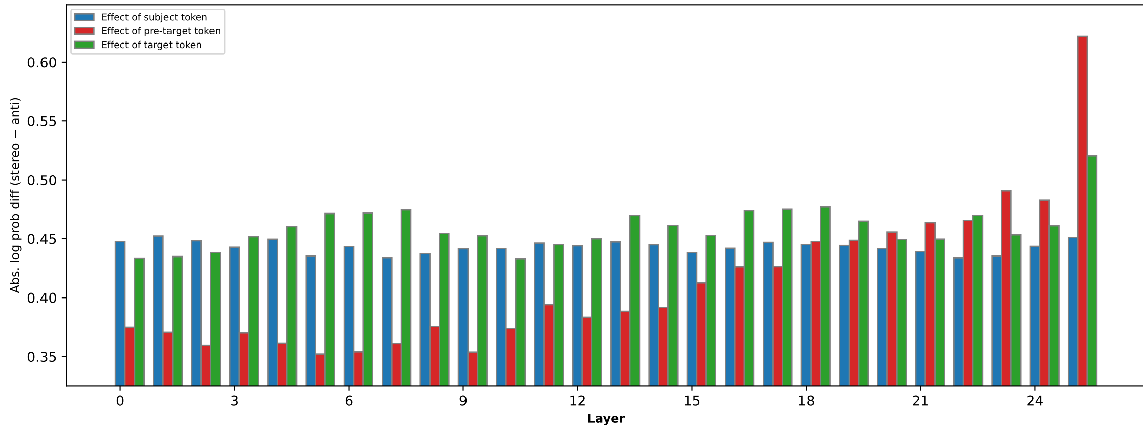
Gender — Gemma-3 1B Post → Pre Instruct activations patched into base model
