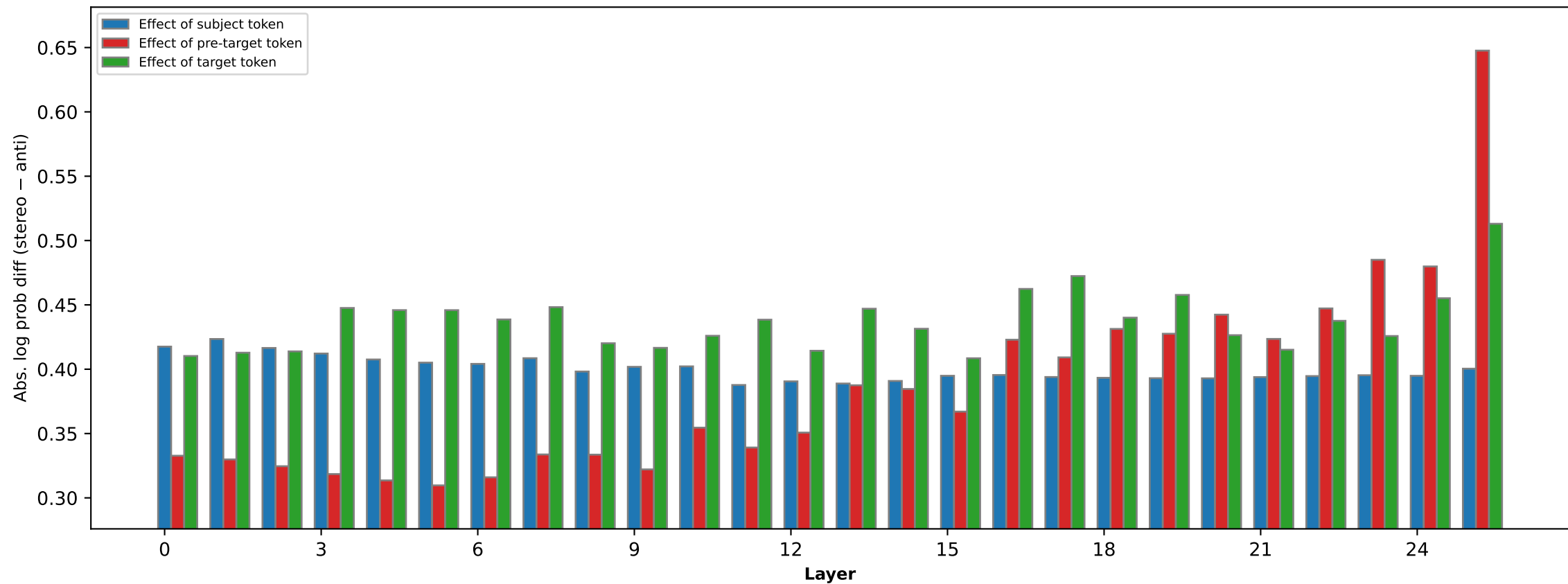
Race — Gemma-3 1B Post → Pre Instruct activations patched into base model
