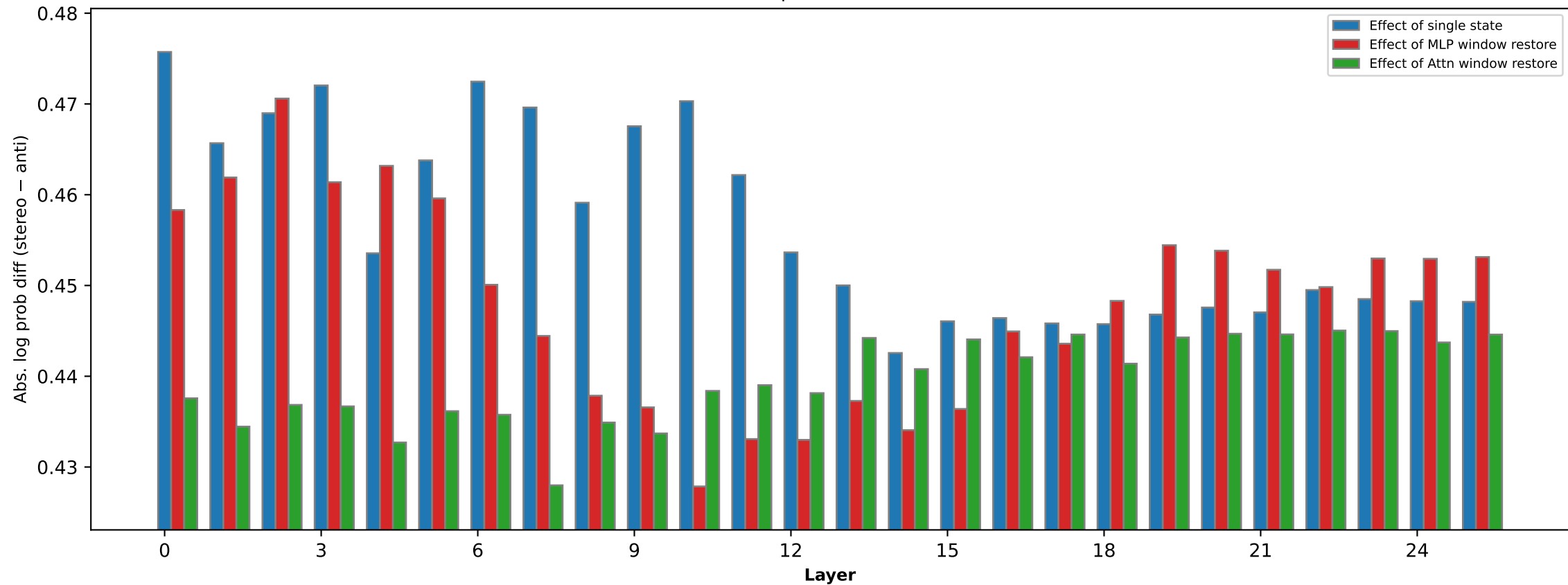
Gender — Gemma-3 1B Pre → Post Base activations patched into instruct model
