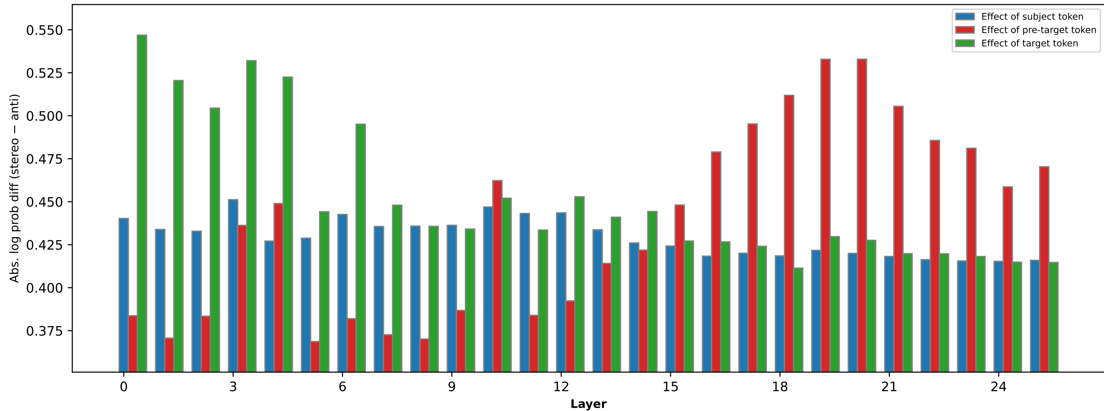
Profession — Gemma-3 1B Pre → Post Base activations patched into instruct model
