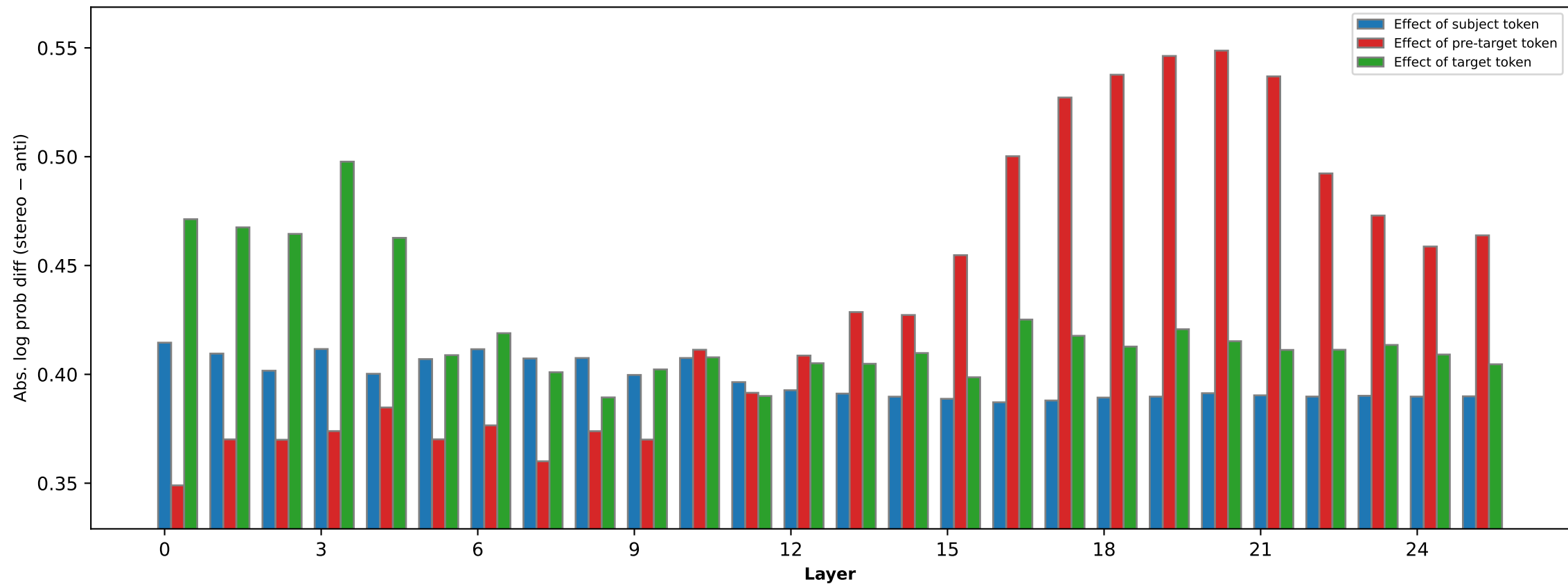
Race — Gemma-3 1B Pre → Post Base activations patched into instruct model
