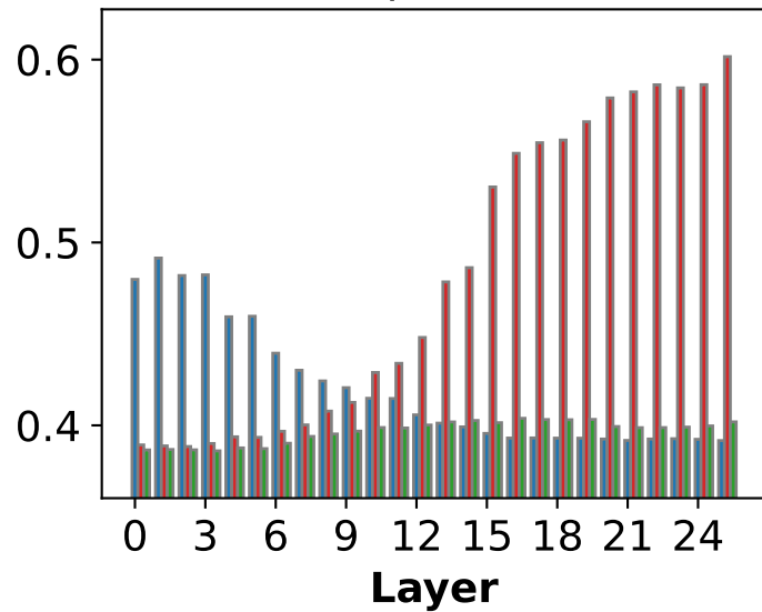
(b) gemma-3-1b-it (post)
