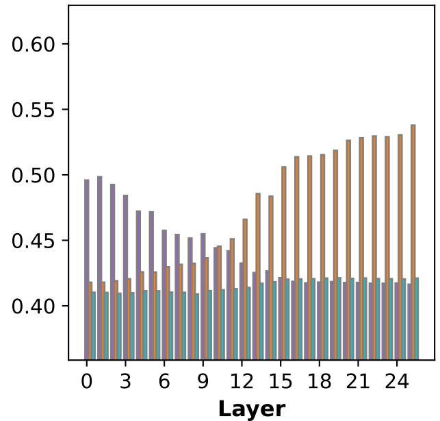
(l) Profession bias effect of different words (gemma-3-1b-it)
