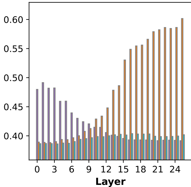
(k) Race bias effect of different words (gemma-3-1b-it)
