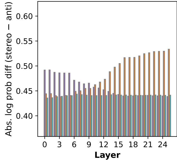
(g) Gender bias effect of states (gemma-3-1b-it)
