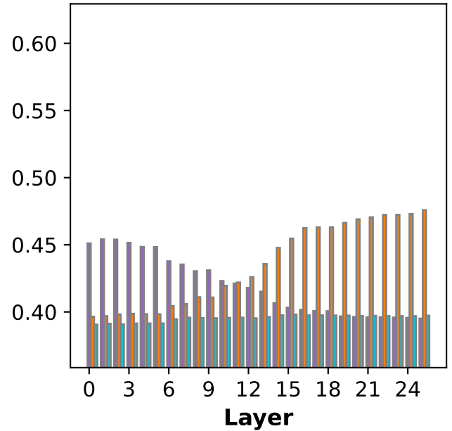
(i) Profession bias effect of states (gemma-3-1b-it)
