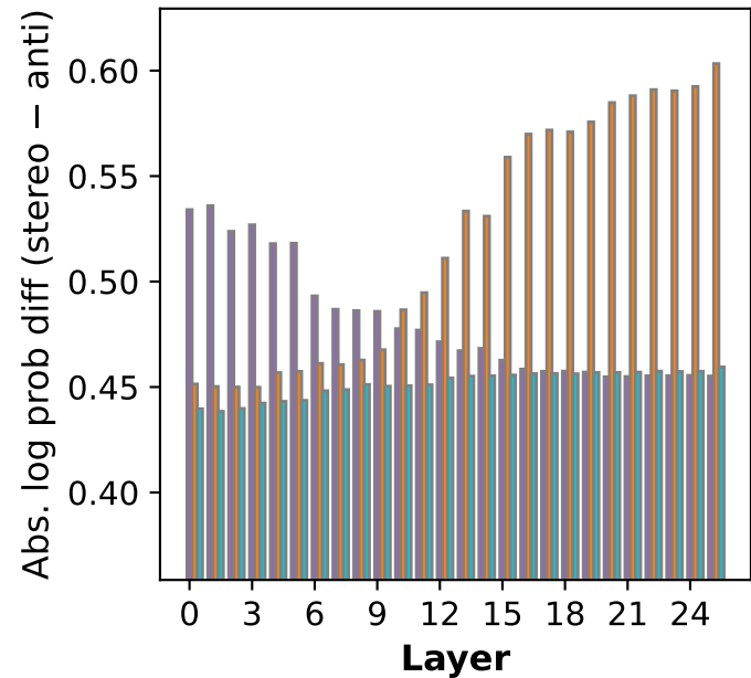
(j) Gender bias effect of different words (gemma-3-1b-it)
