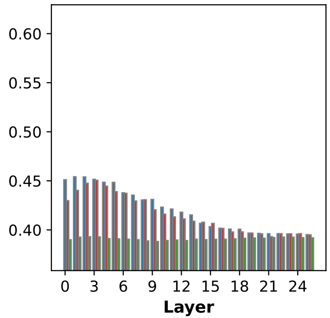
(f) Profession bias effect of different words (gemma-3-1b-pt)
