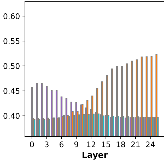
(h) Race bias effect of states (gemma-3-1b-it)
