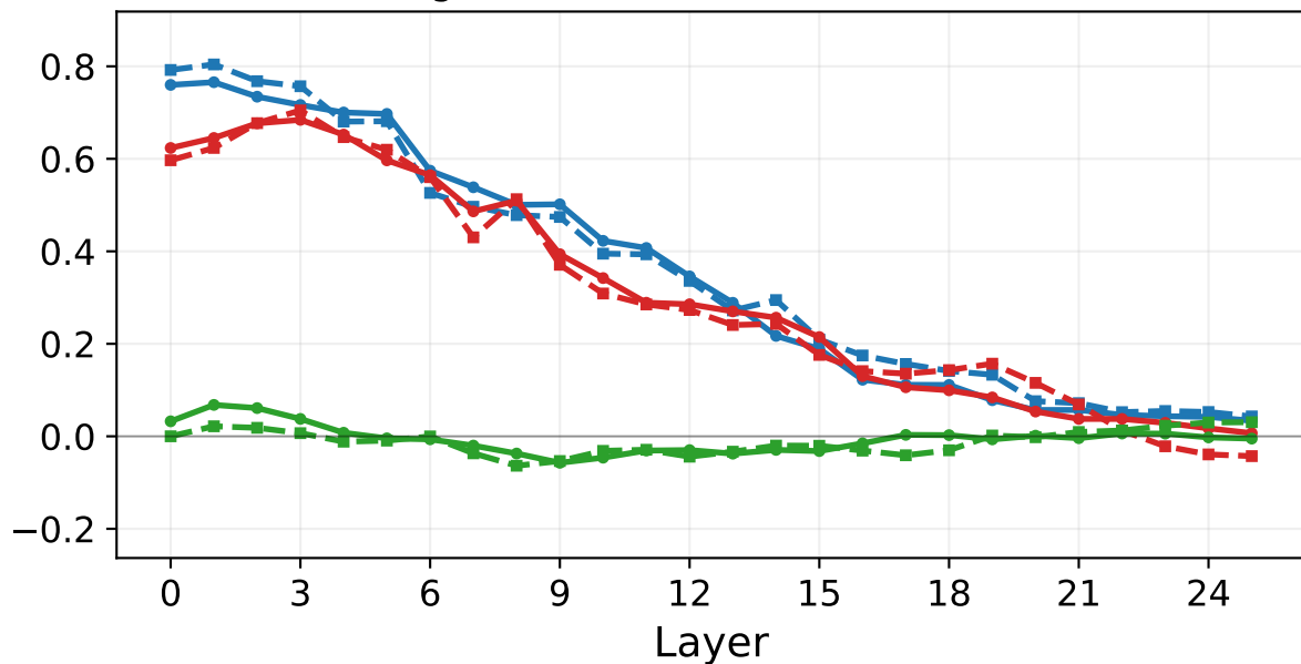
(a) Gender — gemma-3-1b-pt (Pre) solid vs gemma-3-1b-it (Post) dashed
