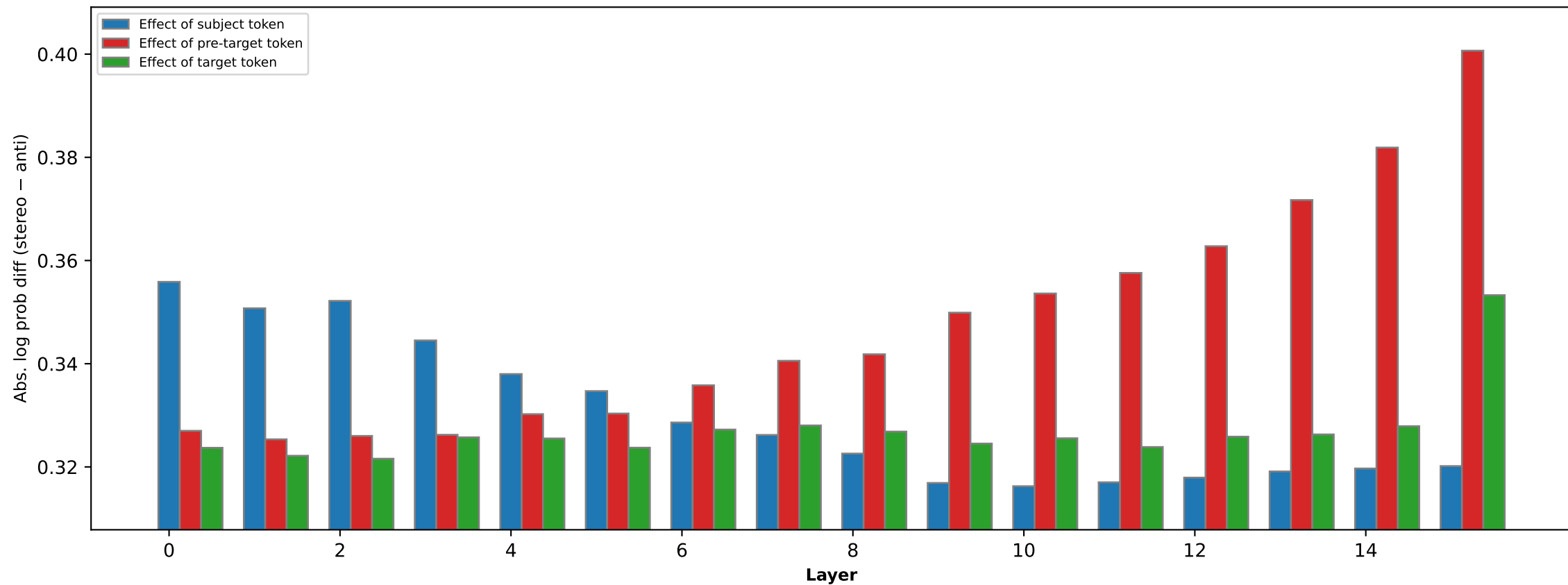
Gender — Llama-3.2 1B Post → Pre Instruct activations patched into base model
