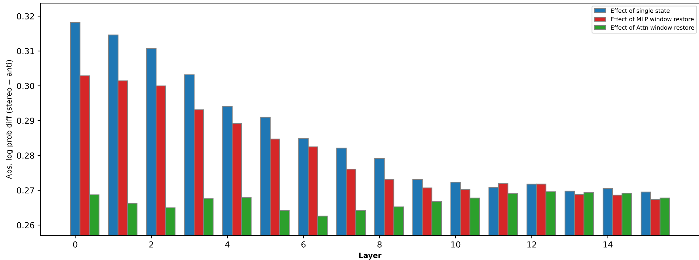
Profession — Llama-3.2 1B Post → Pre Instruct activations patched into base model
