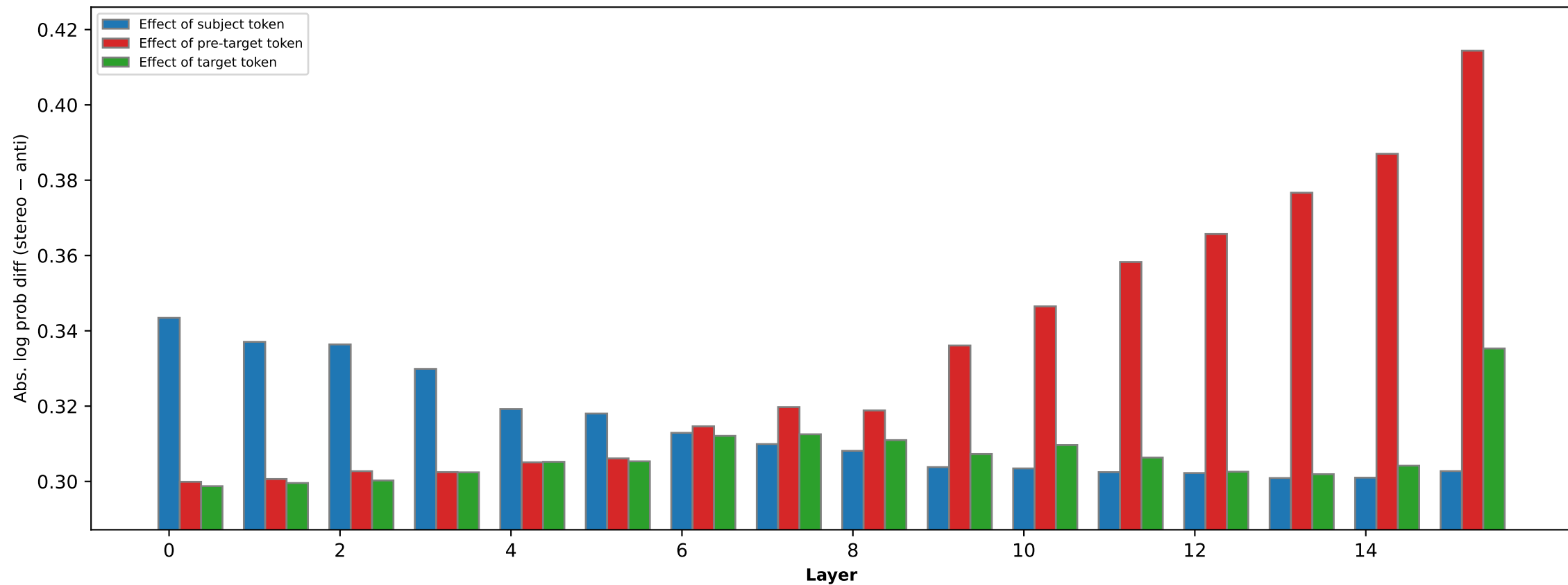
Race — Llama-3.2 1B Post → Pre Instruct activations patched into base model
