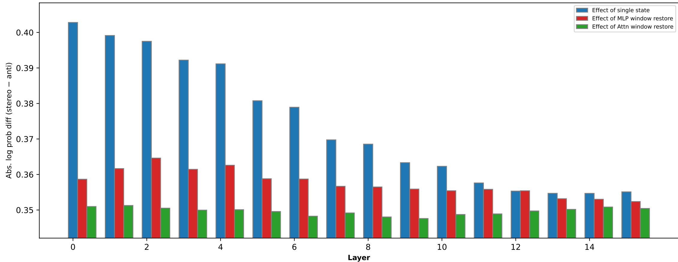
Gender bias effect of states (OLMo-2-0425-1B-Instruct [step1400])
