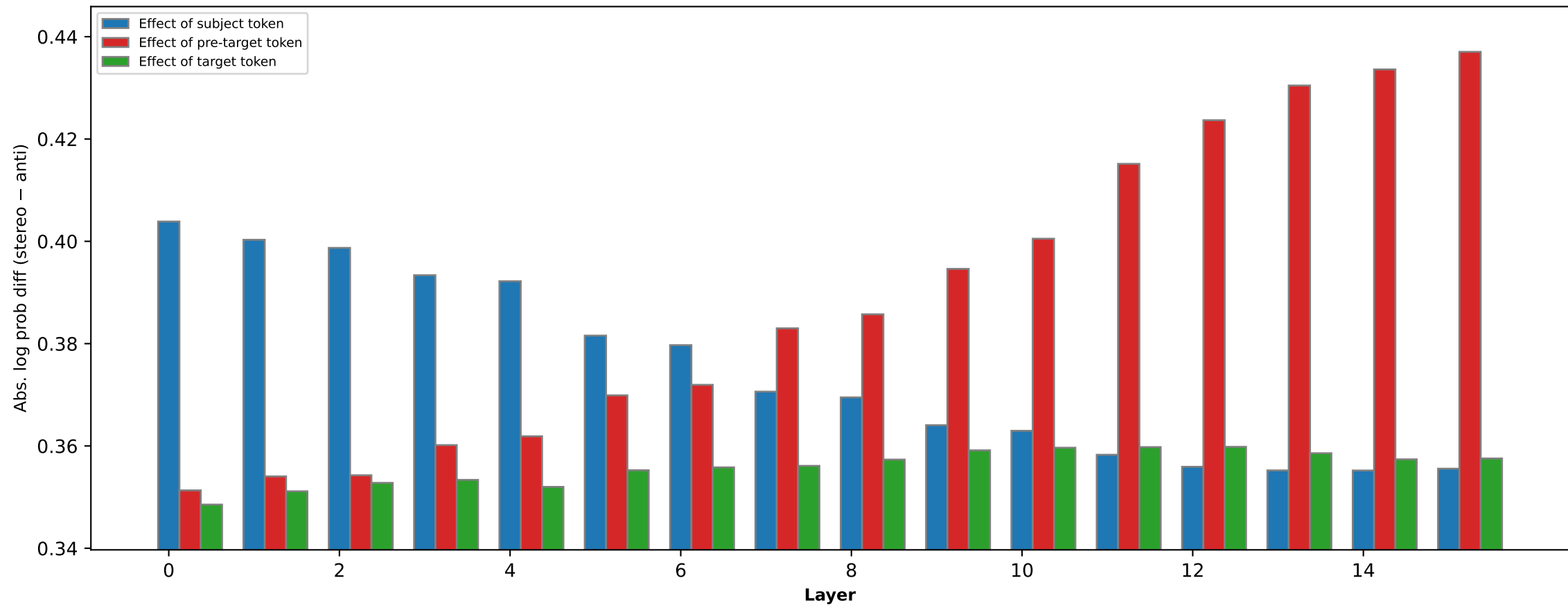
Gender bias effect of different words (OLMo-2-0425-1B-Instruct [step2600])
