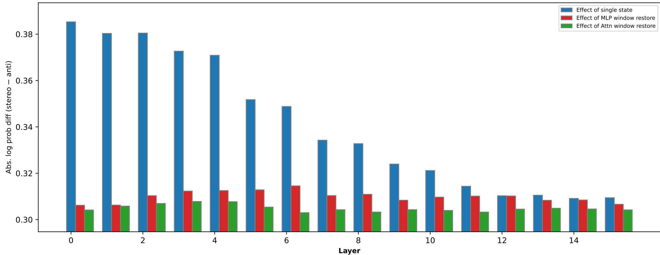
Profession bias effect of states (OLMo-2-0425-1B-Instruct [step2600])
