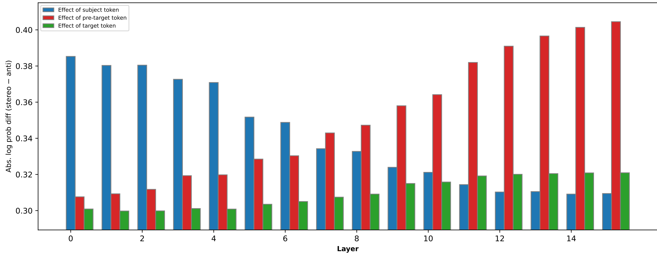
Profession bias effect of different words (OLMo-2-0425-1B-Instruct [step2600])
