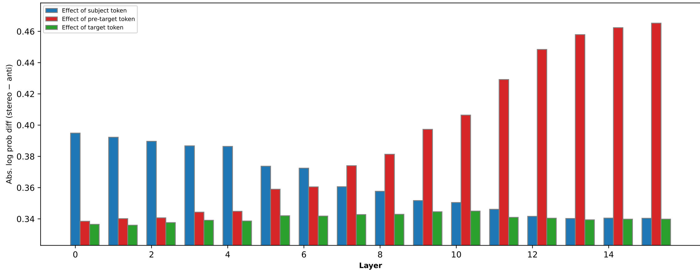
Race bias effect of different words (OLMo-2-0425-1B-Instruct [step2600])
