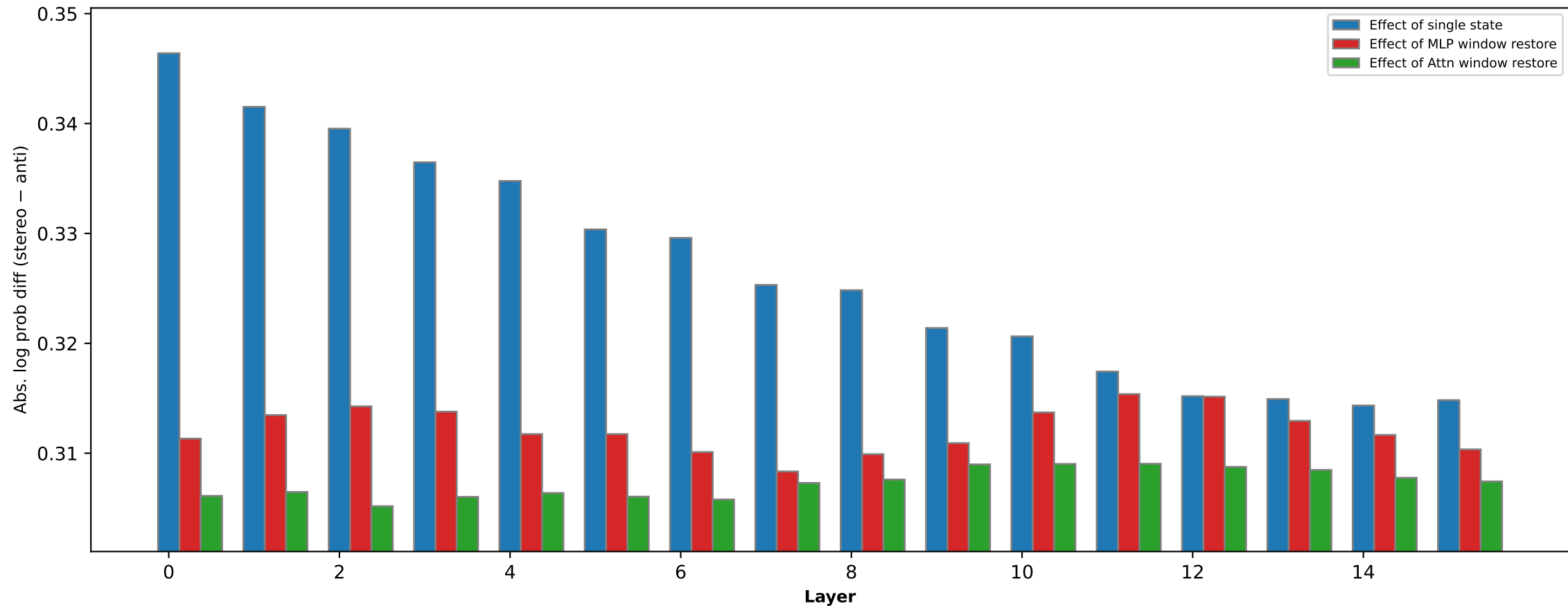
Gender bias effect of states (OLMo-2-0425-1B [2.4T])
