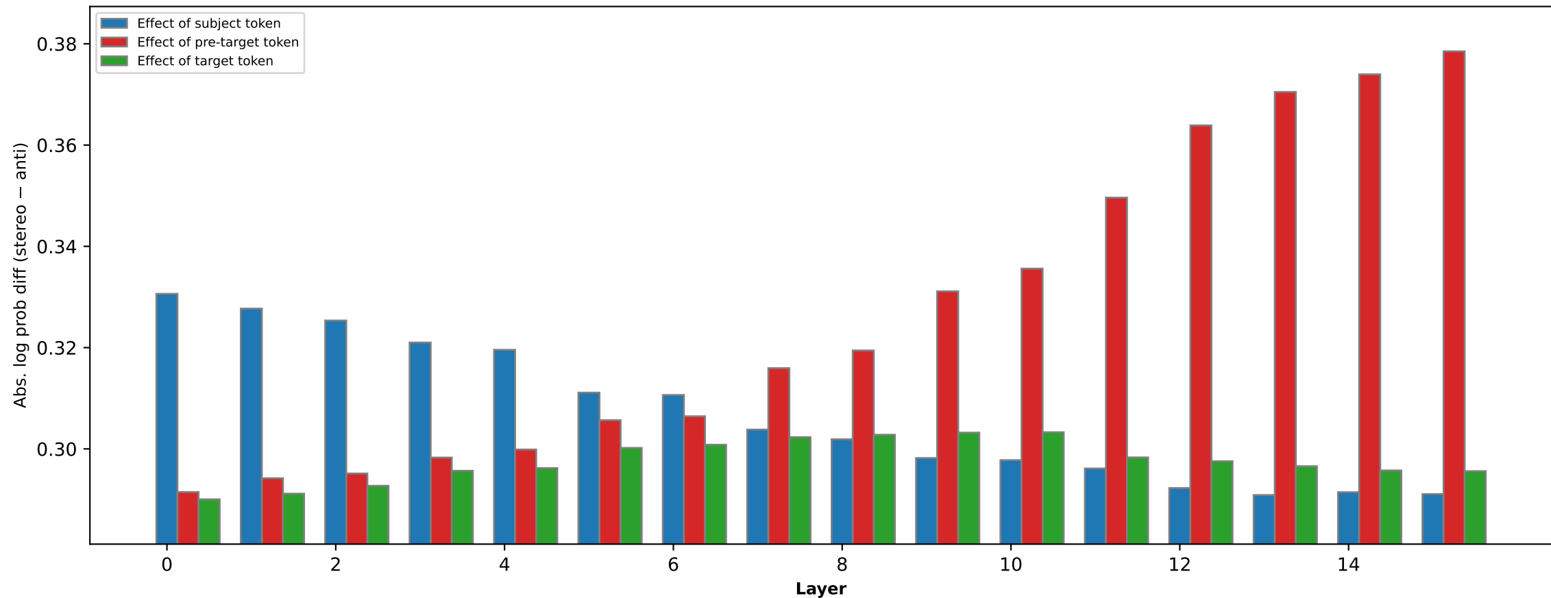
Race bias effect of different words (OLMo-2-0425-1B [2.4T])
