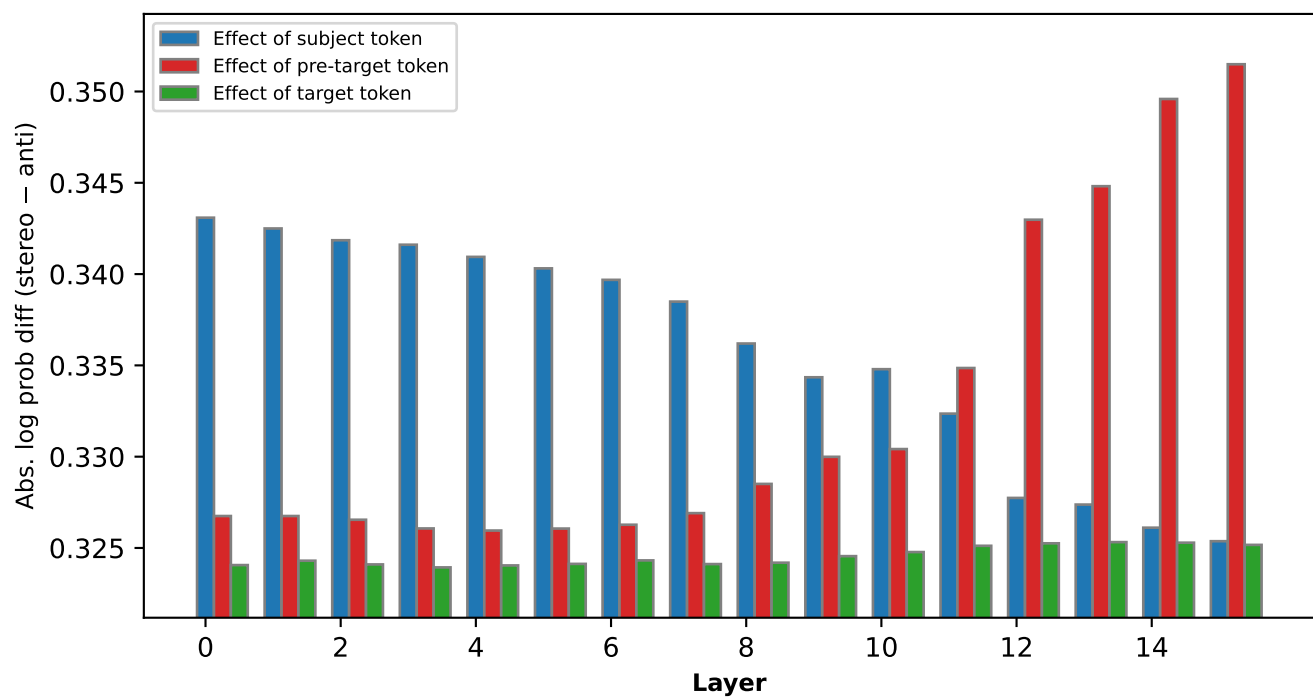
Gender bias effect of different words — OLMo-2-0425-1B (all checkpoints)
