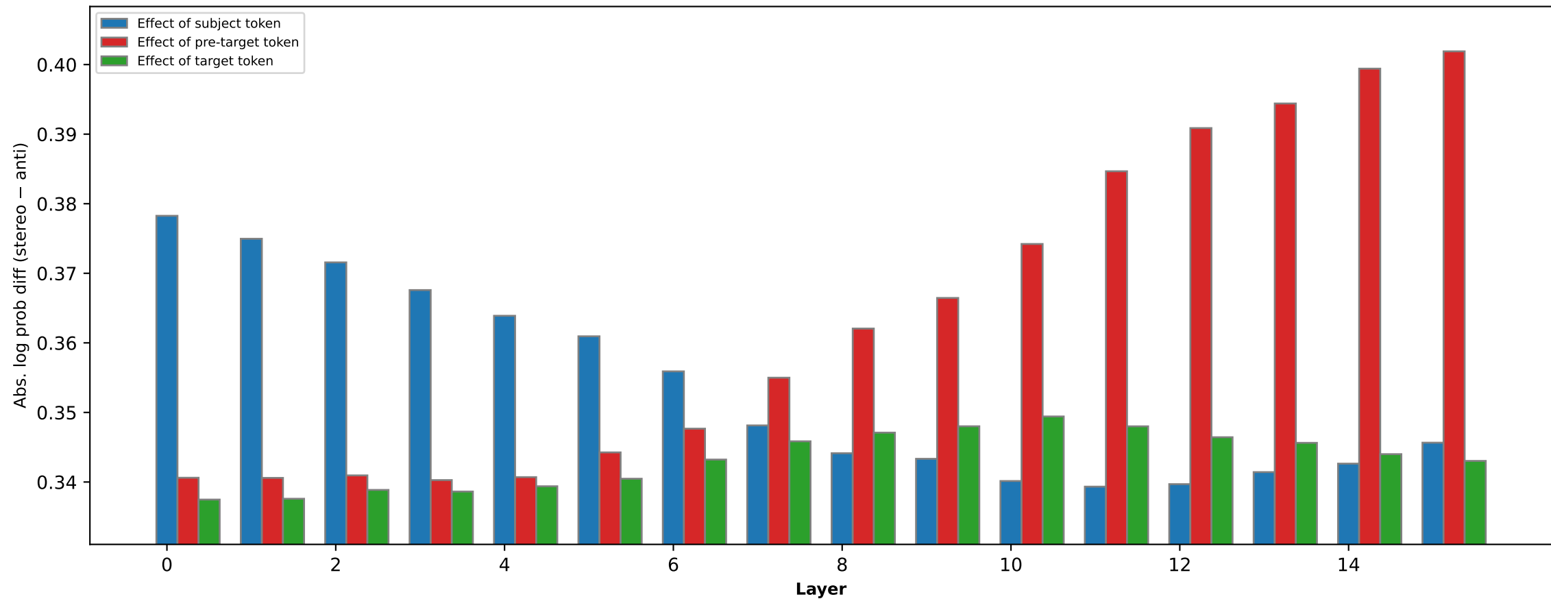
Gender bias effect of different words (OLMo-2-0425-1B [main])
