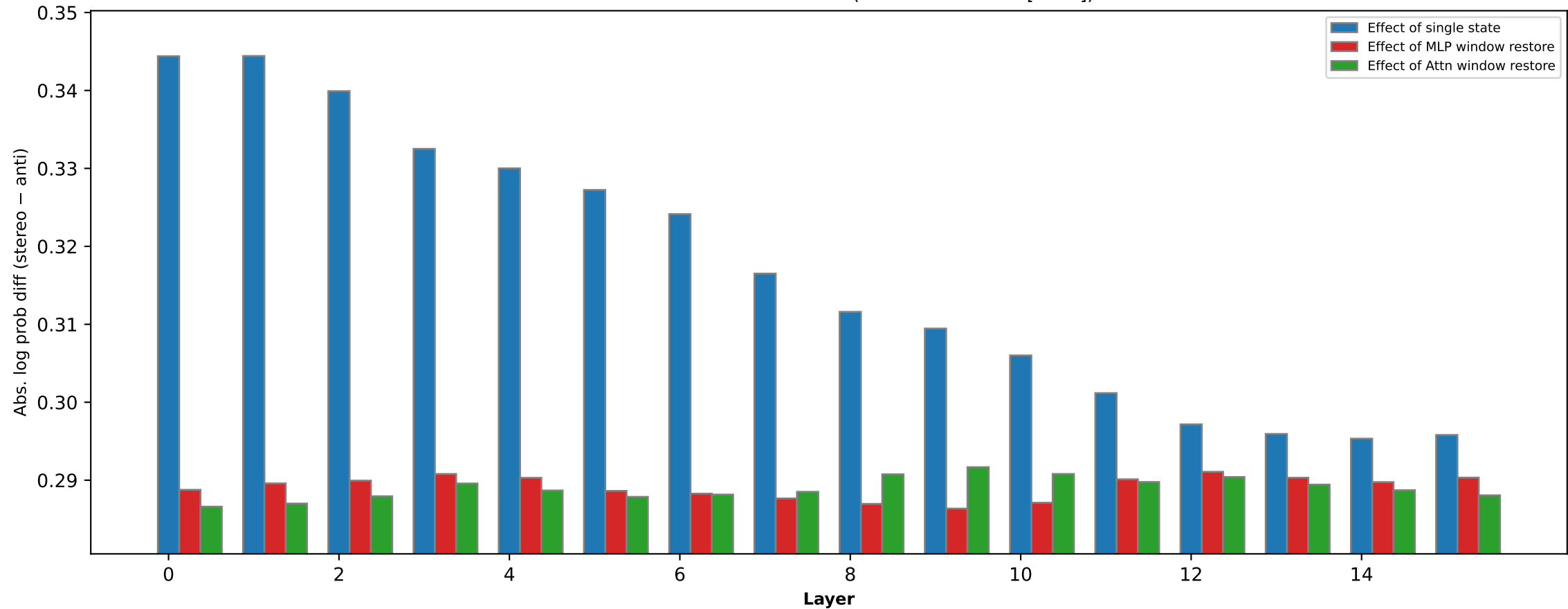
Profession bias effect of states (OLMo-2-0425-1B [main])
