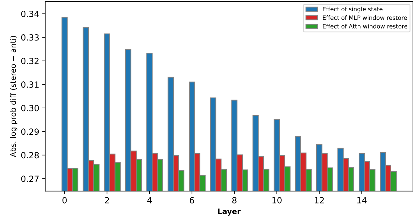
s2-51B
