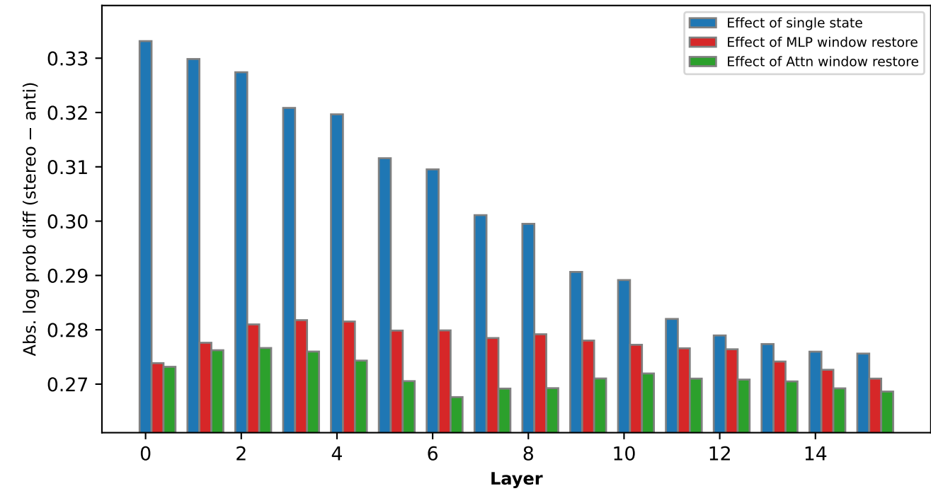
s2-51B
