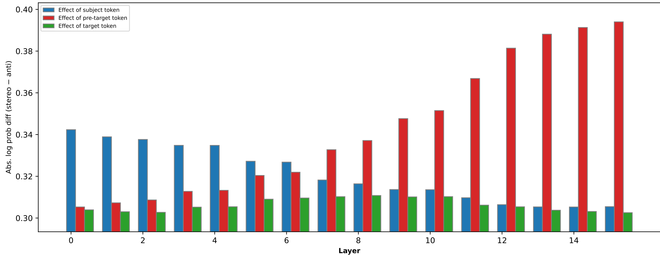
Race bias effect of different words (OLMo-2-0425-1B [s2-3B])
