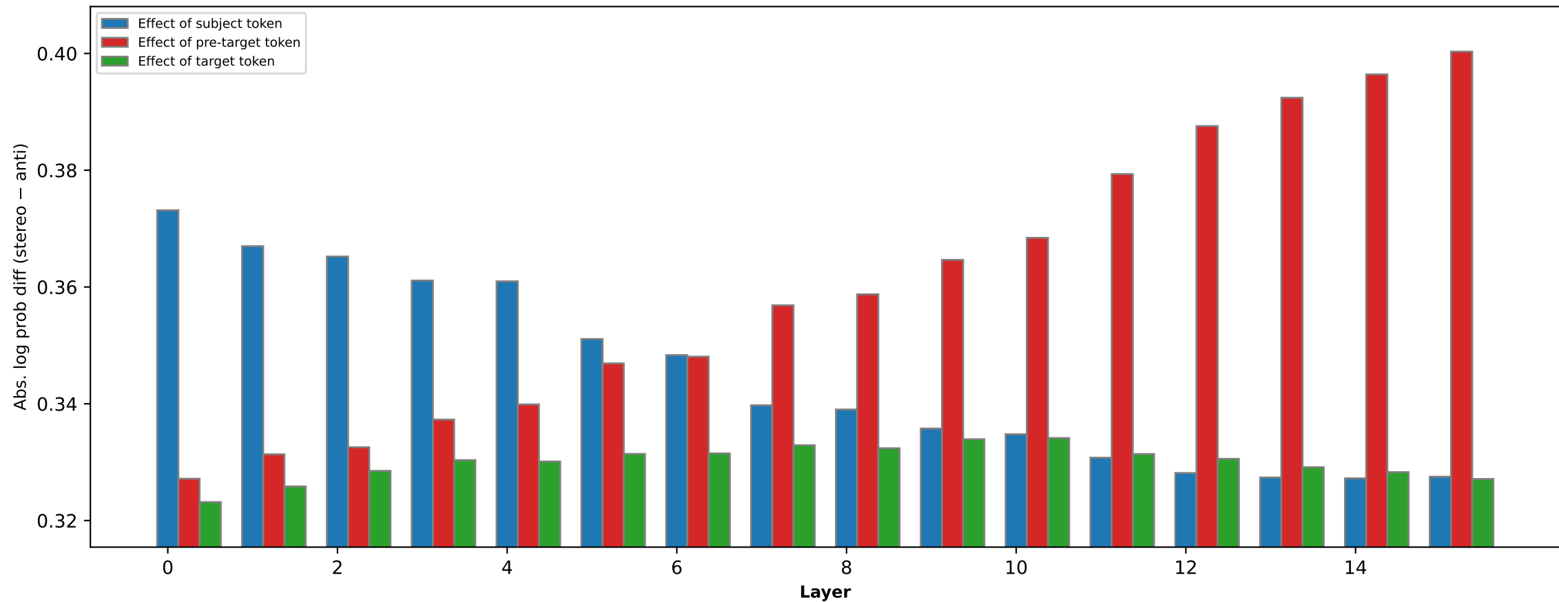
Gender bias effect of different words (OLMo-2-0425-1B [s2-51B])
