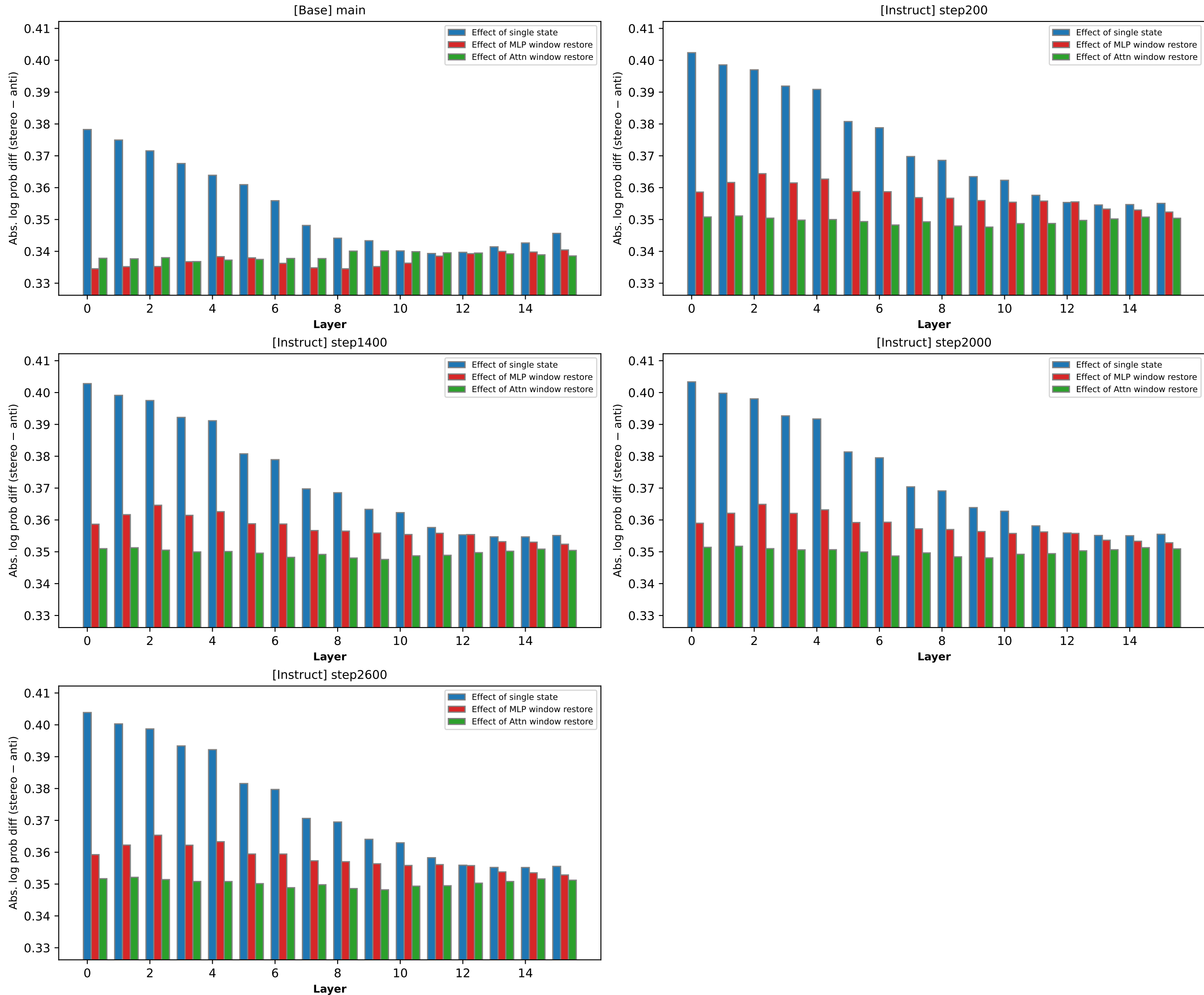
OLMo-2-0425-1B — Gender bias: Base vs. Instruct Abs. log prob diff per layer (blue = States, red = MLP window, green = Attn window) Y-axis fixed across all subplots.
