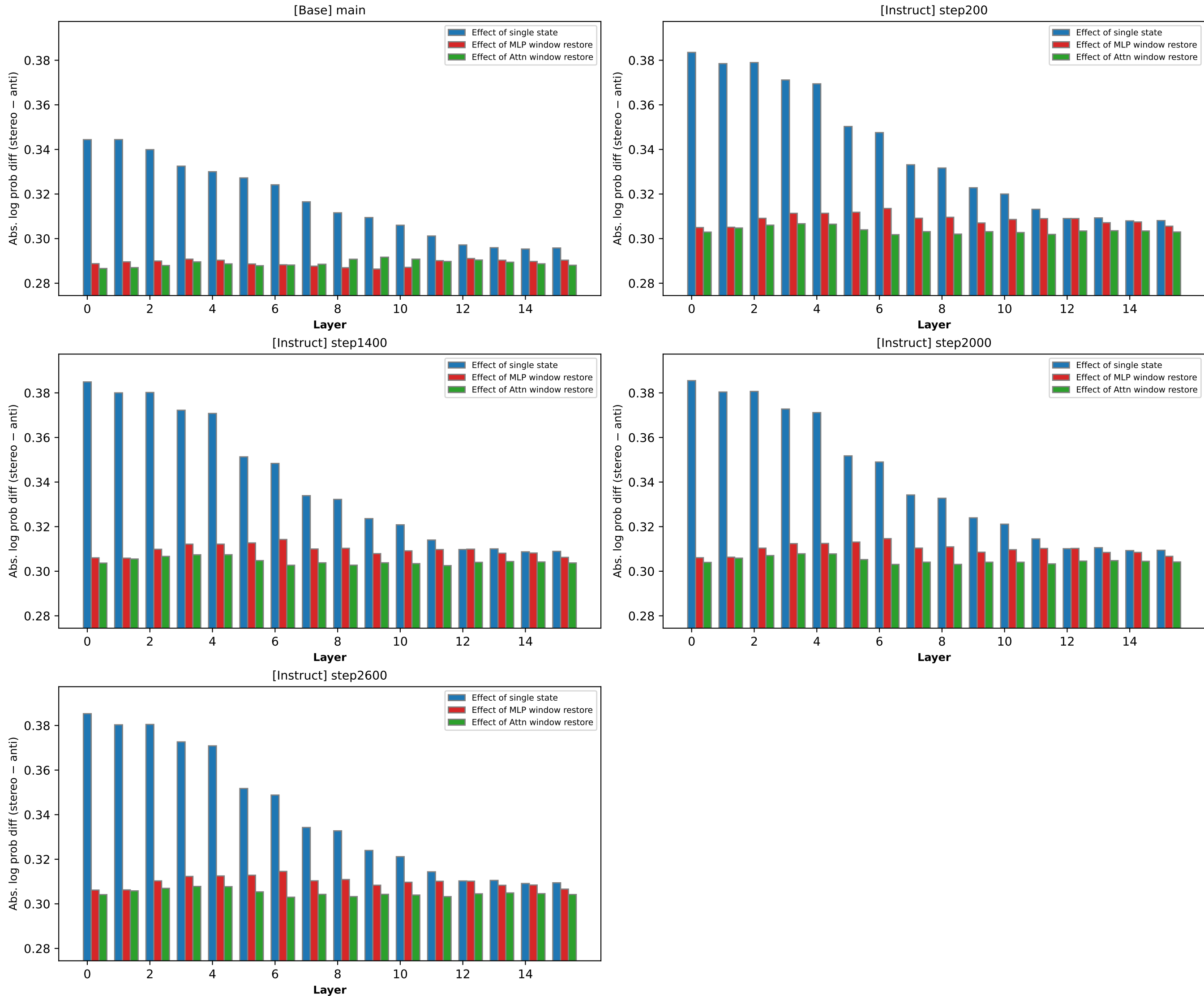
OLMo-2-0425-1B — Profession bias: Base vs. Instruct Abs. log prob diff per layer (blue = States, red = MLP window, green = Attn window) Y-axis fixed across all subplots.
