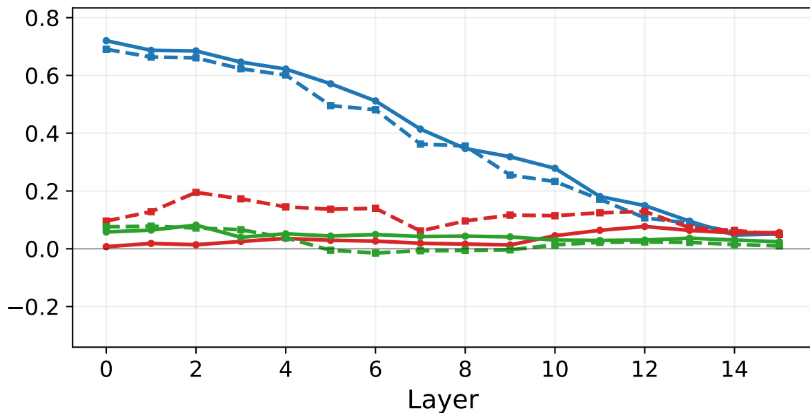
(a) Gender — OLMo-2-0425-1B (Pre) solid vs OLMo-2-0425-1B-Instruct (Post) dashed
