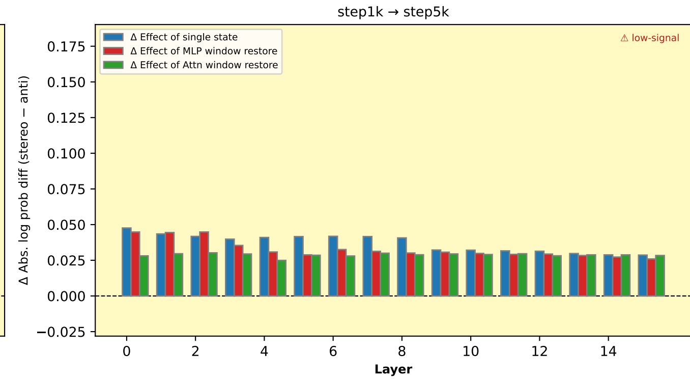
pythia-1b — Gender bias: \Delta per layer vs. previous checkpoint Bars show change in abs. log prob diff (curr – prev) at each layer. Positive = more causal effect acquired. Y-axis fixed across all intervals.
