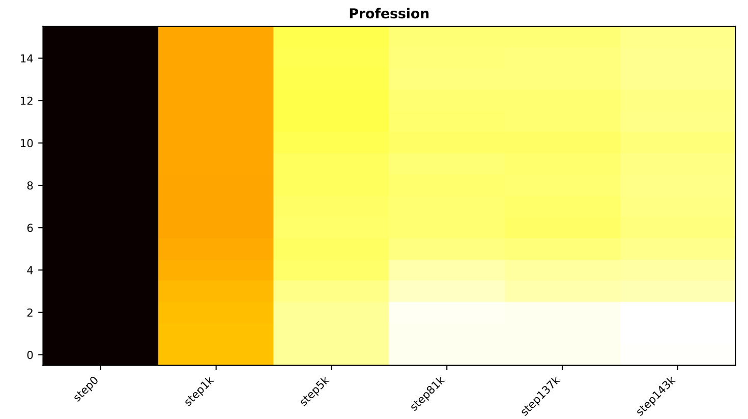
pythia-1b | Causal Tracing — Mean Indirect Effect X: Training Checkpoint Y: Layer Colour: peak-window mean score
