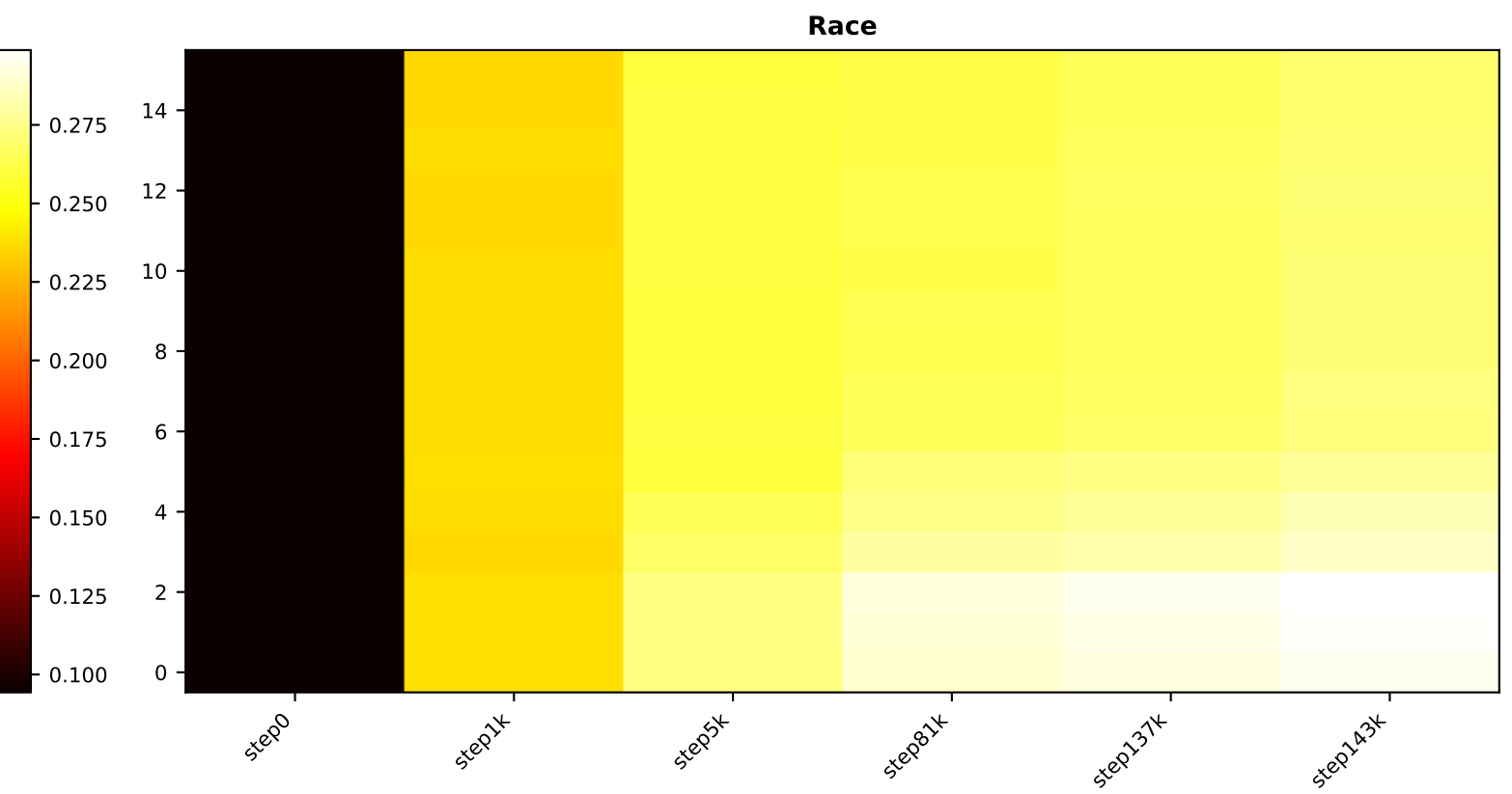
pythia-1b | Causal Tracing — Mean Indirect Effect X: Training Checkpoint Y: Layer Colour: peak-window mean score
