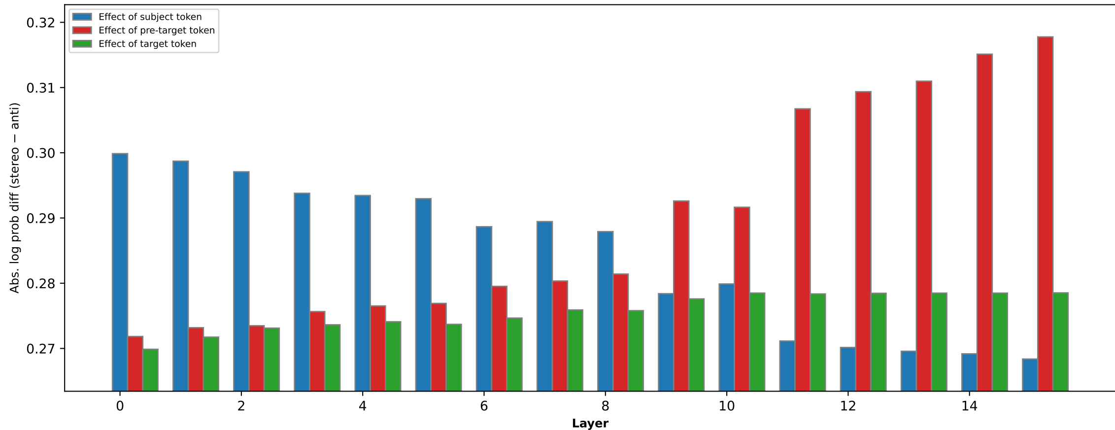
Profession bias effect of different words (pythia-1b [step137k])
