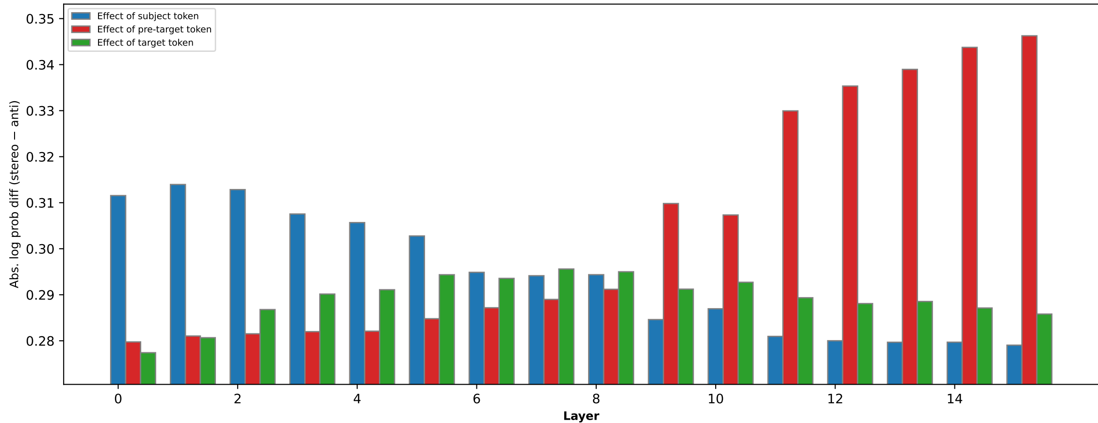
Race bias effect of different words (pythia-1b [step143k])
