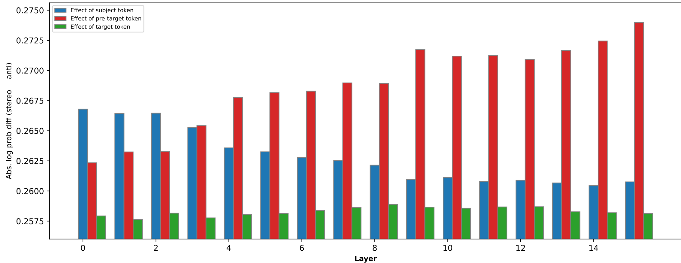
Gender bias effect of different words (pythia-1b [step1k])
