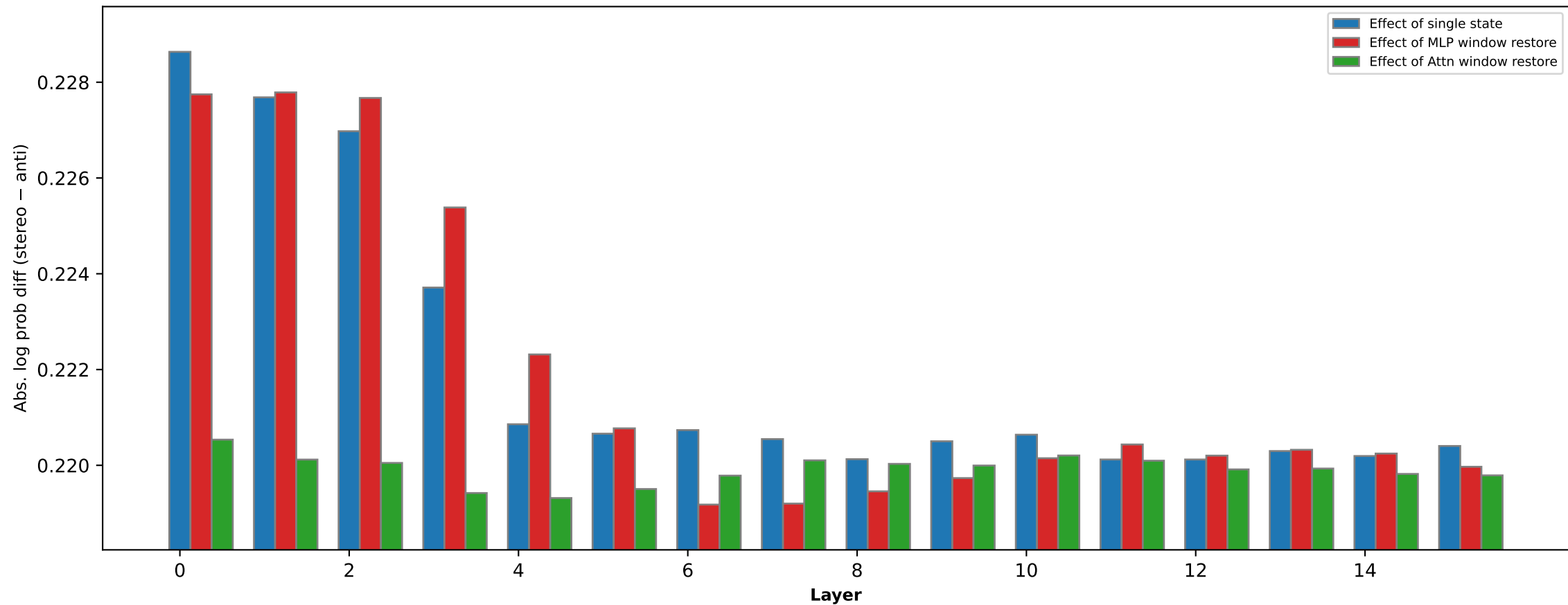
Profession bias effect of states (pythia-1b [step1k])
