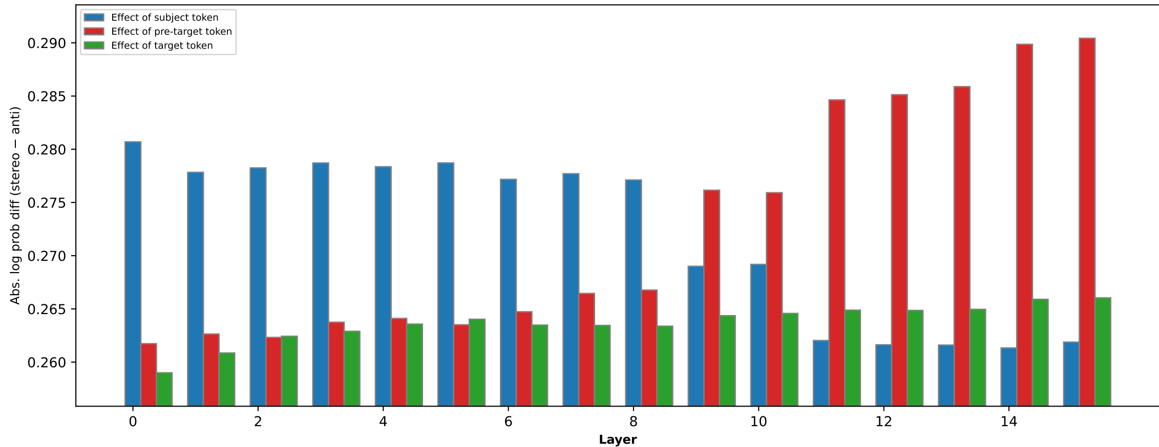
Profession bias effect of different words (pythia-1b [step5k])
