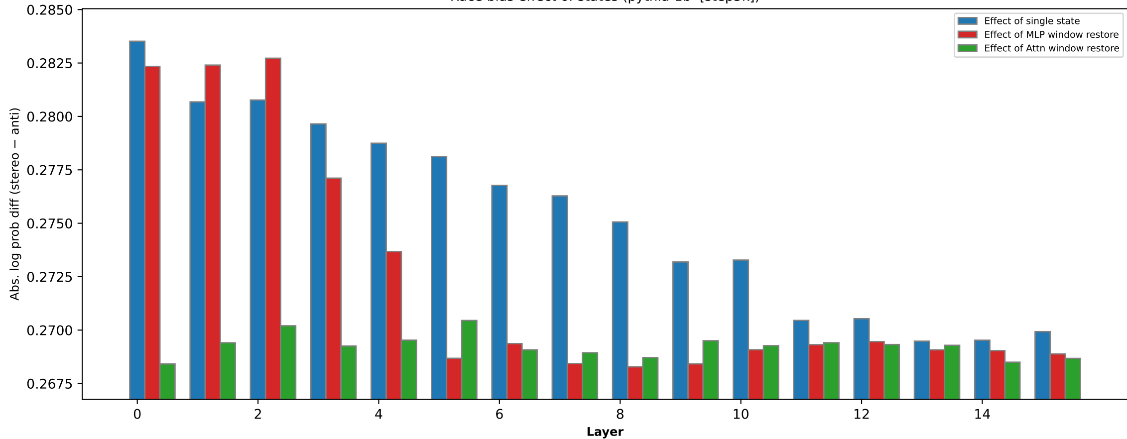
Race bias effect of states (pythia-1b [step5k])
