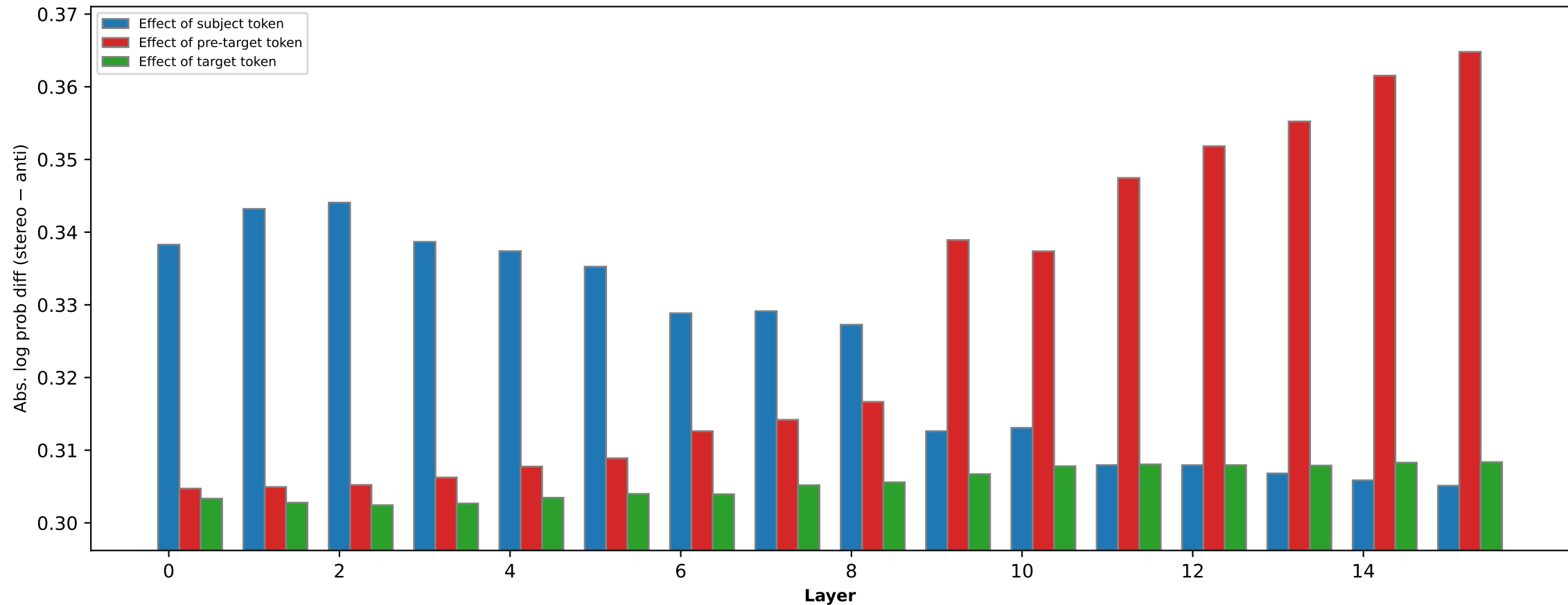
Gender bias effect of different words (pythia-1b [step81k])
