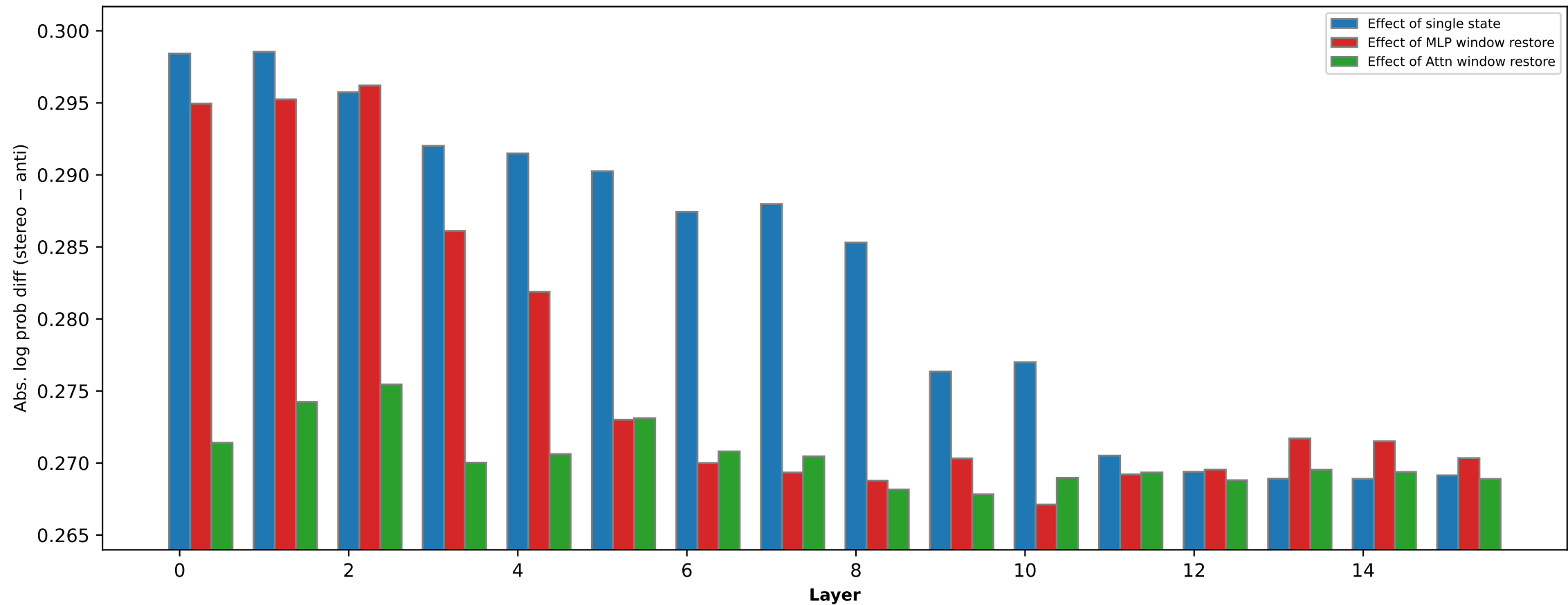
Profession bias effect of states (pythia-1b [step81k])
