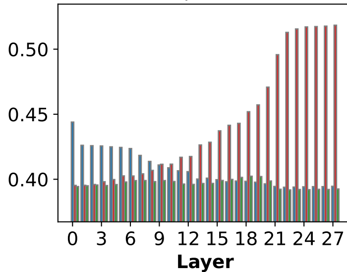
(b) Qwen2.5-1.5B-Instruct (post)
