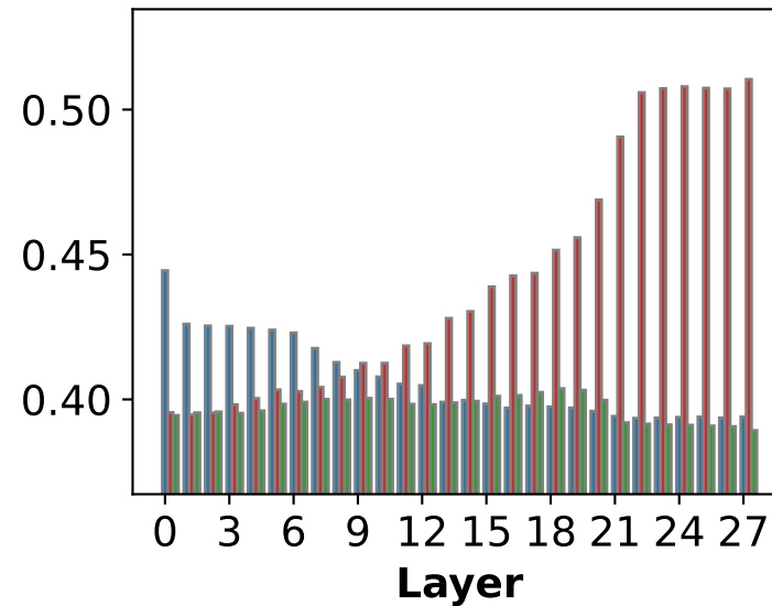
(c) Pre \rightarrow Post
