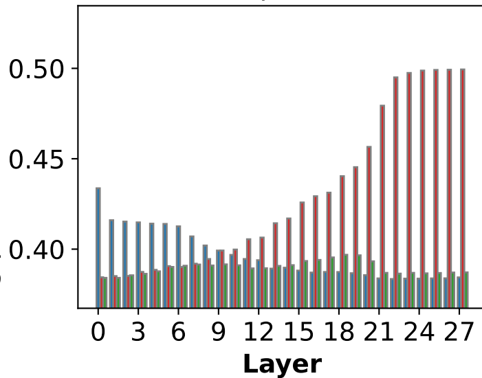
(a) Qwen2.5-1.5B (pre)
