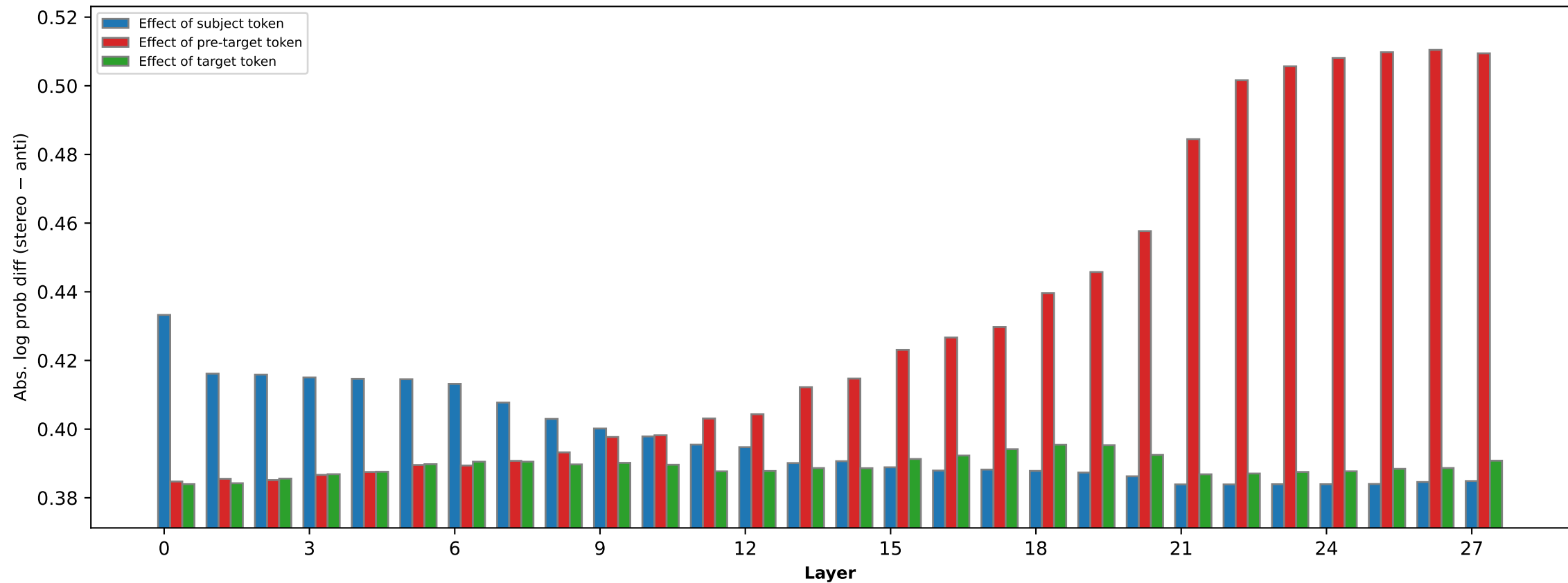
Race — Qwen2.5 1.5B Post → Pre Instruct activations patched into base model
