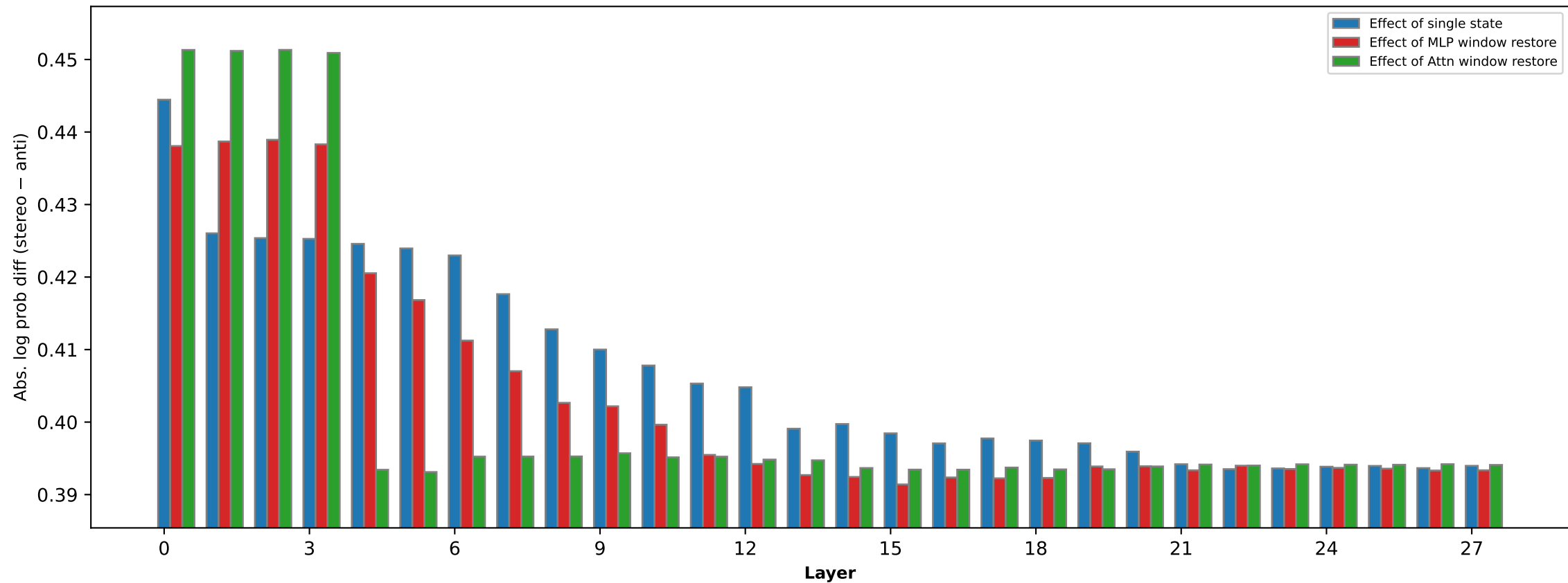
Race — Qwen2.5 1.5B Pre → Post Base activations patched into instruct model
