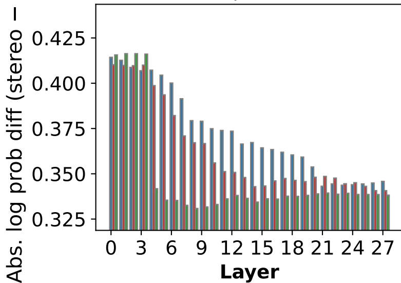
(a) Qwen2.5-1.5B (pre)
