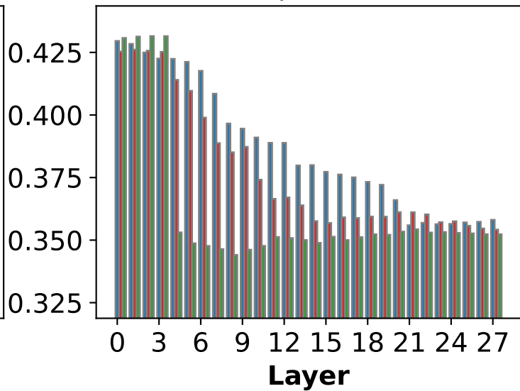
(b) Qwen2.5-1.5B-Instruct (post)
