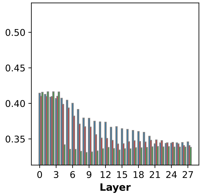
(f) Profession bias effect of different words (Qwen2.5-1.5B)
