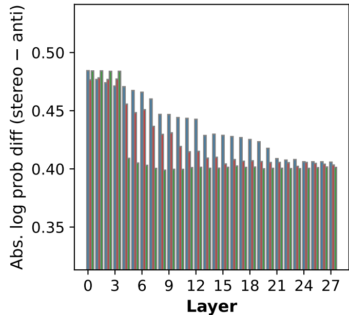
(j) Gender bias effect of different words (Qwen2.5-1.5B-Instruct)
