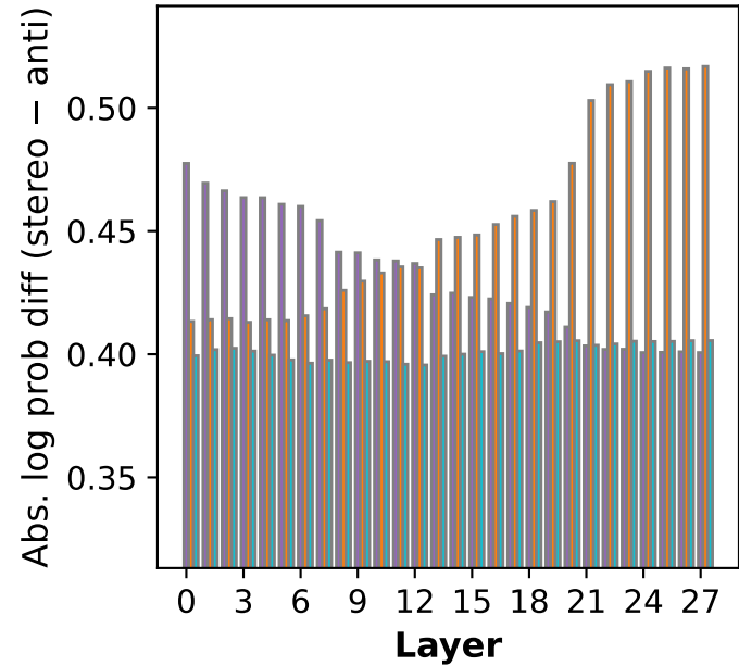
(g) Gender bias effect of states (Qwen2.5-1.5B-Instruct)
