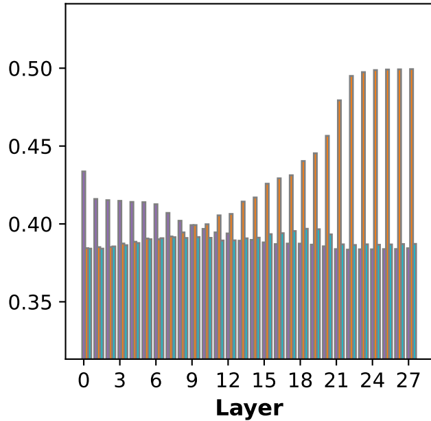
(h) Race bias effect of states (Qwen2.5-1.5B-Instruct)
