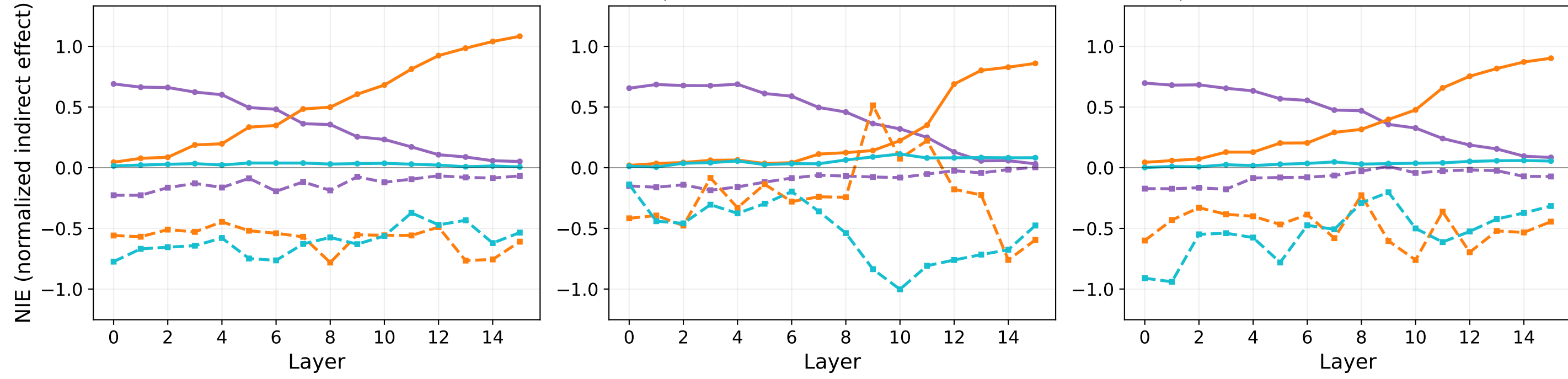
OLMo-2-0425-1B within-model (solid) vs OLMo-2-0425-1B-Instruct cross-patch (dashed) (g) Gender — States NIE (h) Race — States NIE (i) Profession — States NIE
