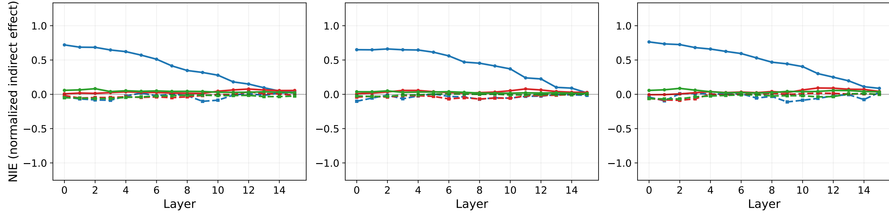
OLMo-2-0425-1B within-model (solid) vs OLMo-2-0425-1B-Instruct cross-patch (dashed) (j) Gender — Words NIE (k) Race — Words NIE (l) Profession — Words NIE
