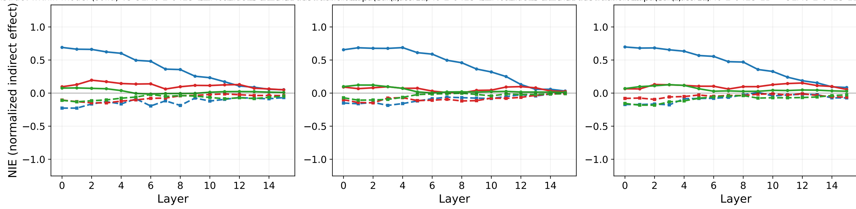
OLMo-2-0425-1B-Instruct within-model (solid) vs OLMo-2-0425-1B-Instruct cross-patch (dashed) (d) Gender — Words NIE (e) Race — Words NIE (f) Profession — Words NIE
