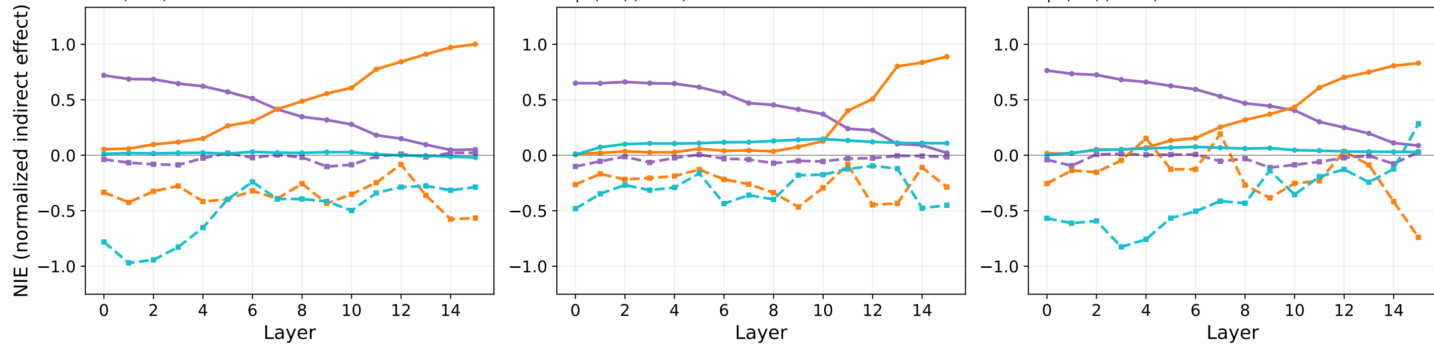
OLMo-2-0425-1B within-model (solid) vs OLMo-2-0425-1B-Instruct cross-patch (dashed) (j) Gender — Words NIE (k) Race — Words NIE (l) Profession — Words NIE
